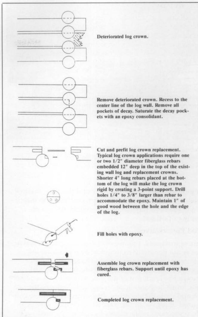
Fig. 21. Epoxy repair. Drawing: Harrison Goodall.
