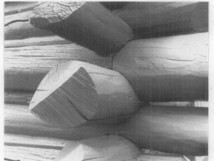
Fig. 20. (a) These deteriorated log crowns were (b) repaired with new crowns which were attached to the historic logs with reinforcing bars and epoxy. Epoxy repair of log crowns is most successful when the repaired crowns are protected from excess moisture by a roof overhang. Photos: Harrison Goodall.
