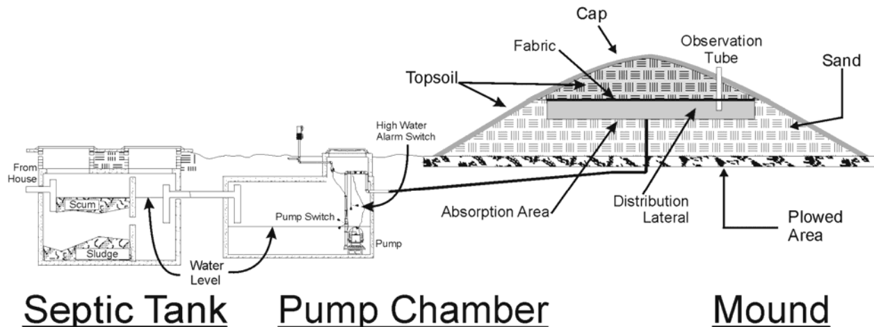
Figure FF-12 Across-section of a septic tank-mound system for on-site disposal
