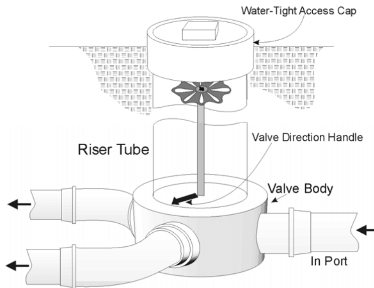
Figure FF-3 Typical Diversion Valve
