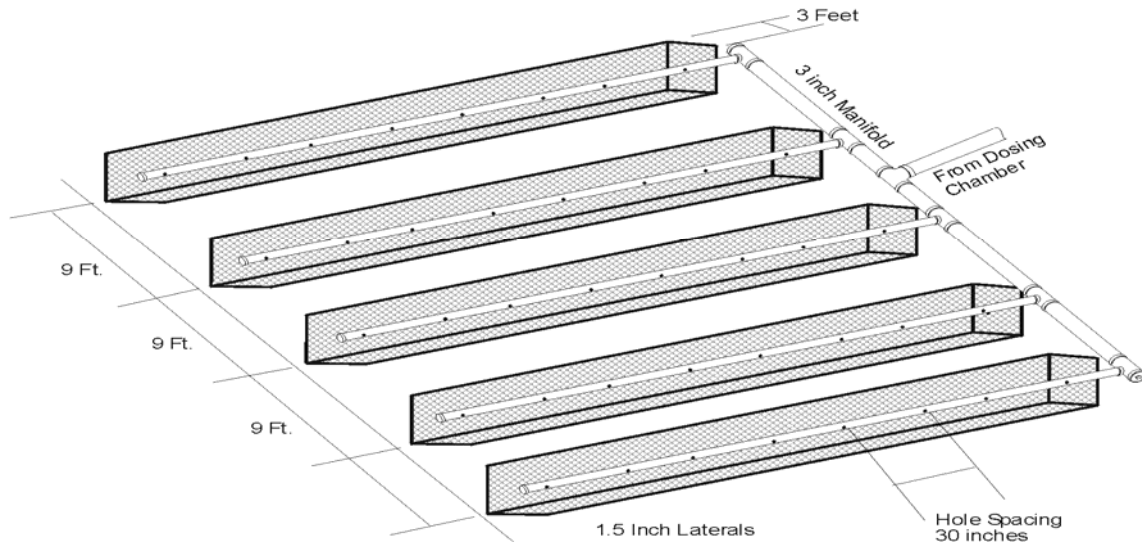
Figure FF-11 Example of a Distribution Network for a Trench System
