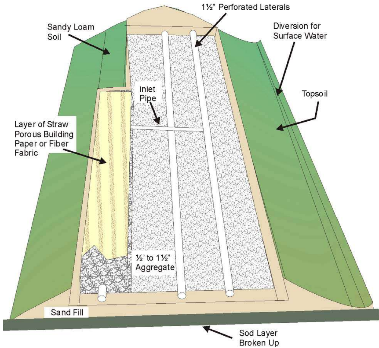
Detailed Schematic of a Mound System
