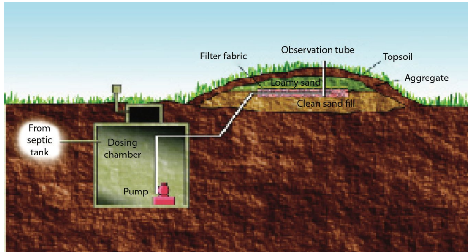
Figure 5: Mound system.
