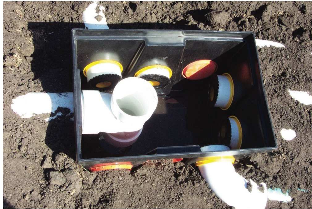
Figure 12: Distribution box.
