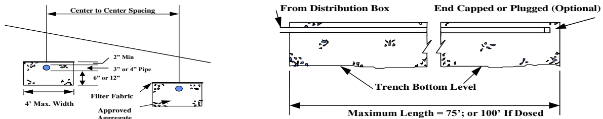
Figure 14 - Leaching Trenches
