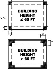
CORNER DEFINITION (SEE NOTES 4, 5 & 6)
