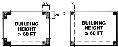
(SEE NOTES 4, 5 & 6) CORNER DEFINITION
