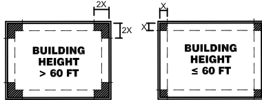
CORNER DEFINITION (SEE NOTES 4, 5 & 6)
