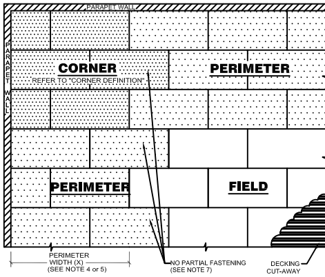
8 FASTENERS (1:4 FT 2 )
