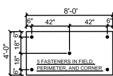
INSULATION FASTENING
