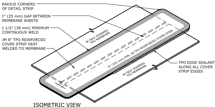
ISOMETRIC VIEW
