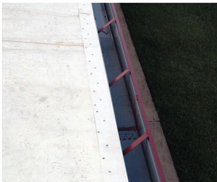
FlexClad™ metal drip edge, properly secured
