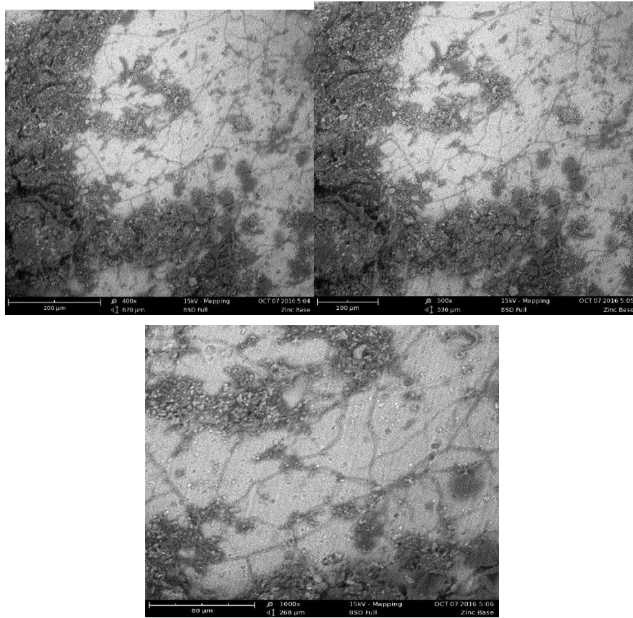
Fig. 13. Scanning Electron Microscope (SEM) Micrographs of dark-black Deposit on Zinc-Coated base roofing sheet at different Magnifications (400X, 500X, 1000X). The light areas have low deposit of the material; the substrate is still shining and the dark areas have large deposit of the material; the substrate is covered.
