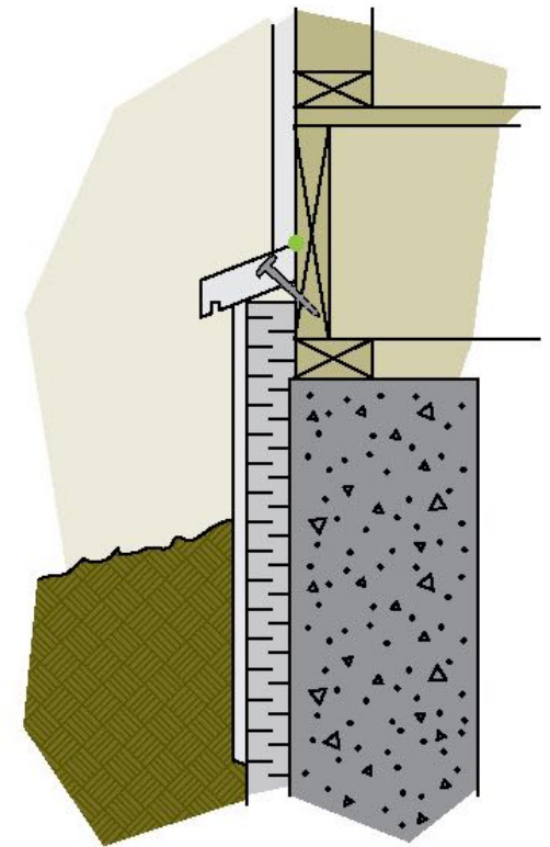
Wood flashing
