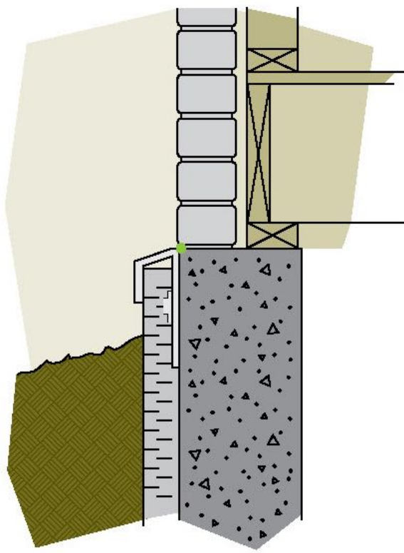
J channel
