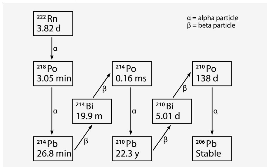
Fig. 7.1. Simplified decay scheme for radon, with isotopes and half-lives
