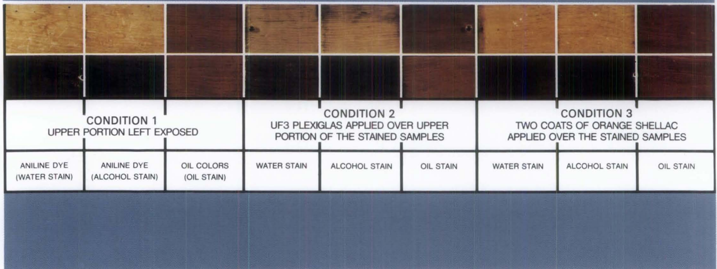
Figure 1. The 10-year test results of the National Park Service's Wood Stain Durability Test are shown. The upper half of the test board was exposed in a window to north light. The bottom was covered during the test period. Comparison of the corresponding exposed and unexposed areas reveals the extreme susceptibility of certain commonly used wood stains to damage by light. Photo: Mike Wiltshire, National Park Service.
