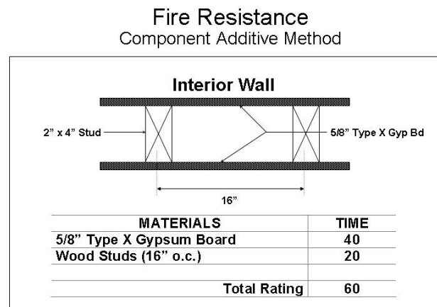
Figure 1. Interior wood stud wall of Example 1
