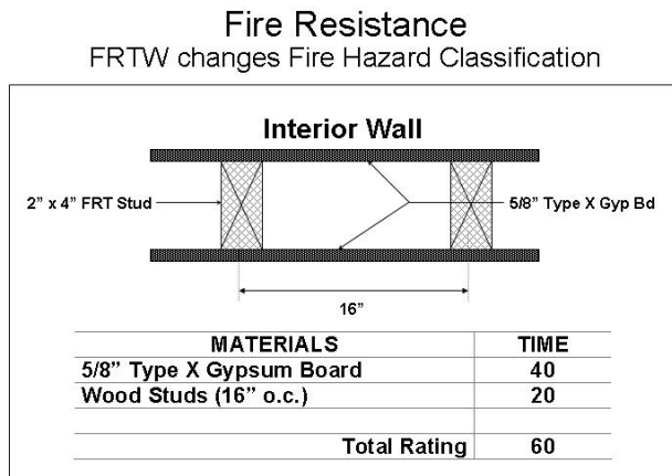
Figure 2. Interior stud wall of Example 1 with FRTW studs
