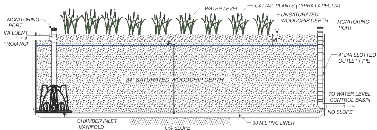
Figure 8. Cross-section Detail of a Typical Vegetated Denitrifying Woodchip Bed
