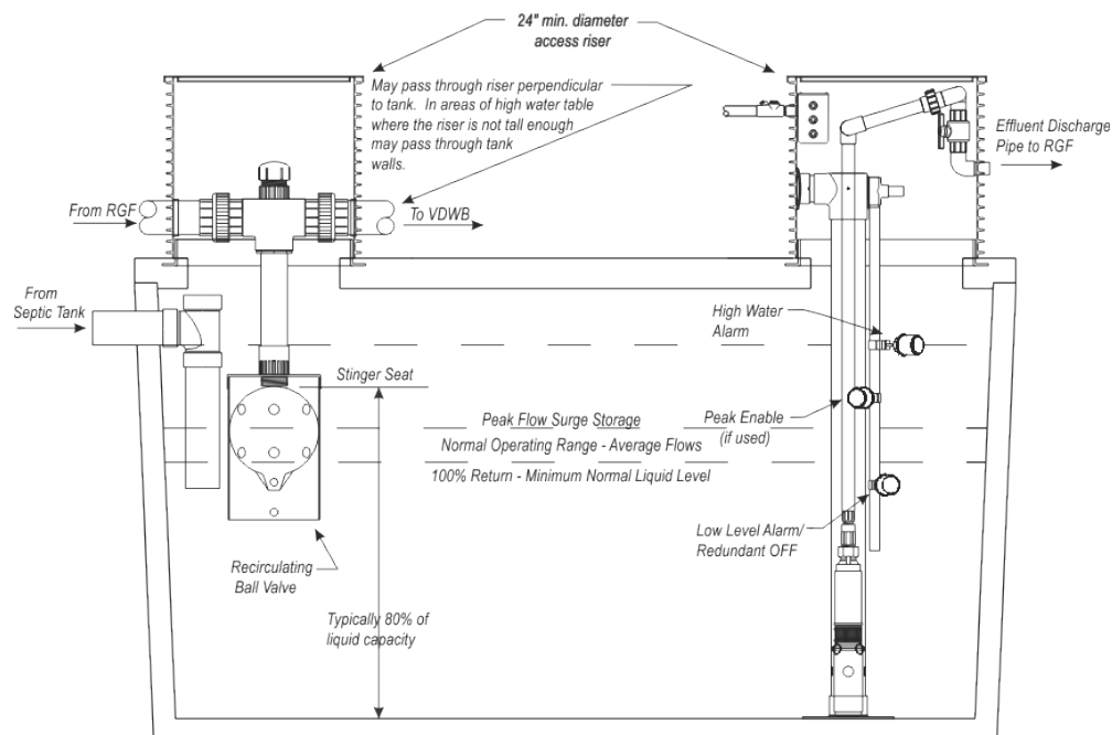
Figure 7. Example of a Recirculating/Mixing Tank with a Recirculating Ball Valve
