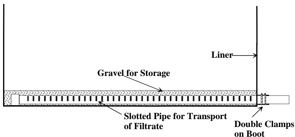
Figure 16. Cross-section of a Basic Recirculating Gravel Filter Underdrain
