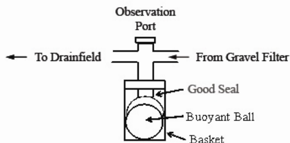
Figure 18. Example of a Recirculating Ball Valve
