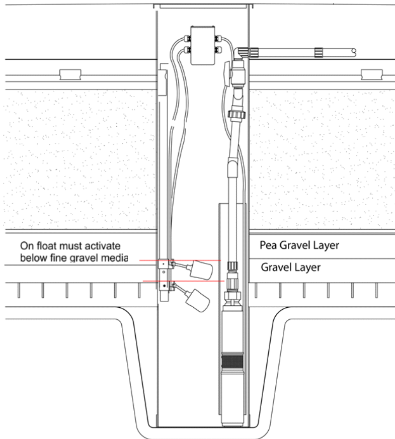
Figure 17. Example of an Internal Pump Basin Assembly (w/ Float Setting Detail)
