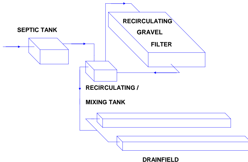
Figure 1. Layout of a Recirculating Gravel Filter
