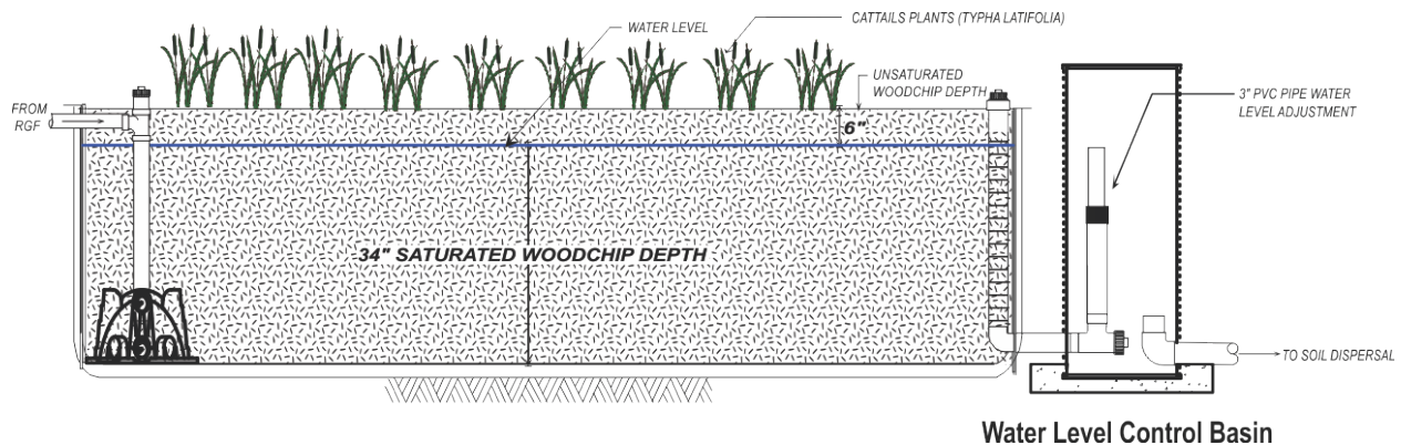
Figure 6. Cross-section of a Typical Vegetated Denitrifying Woodchip Bed
