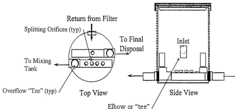
Figure 19 – Example of Splitter Basin
