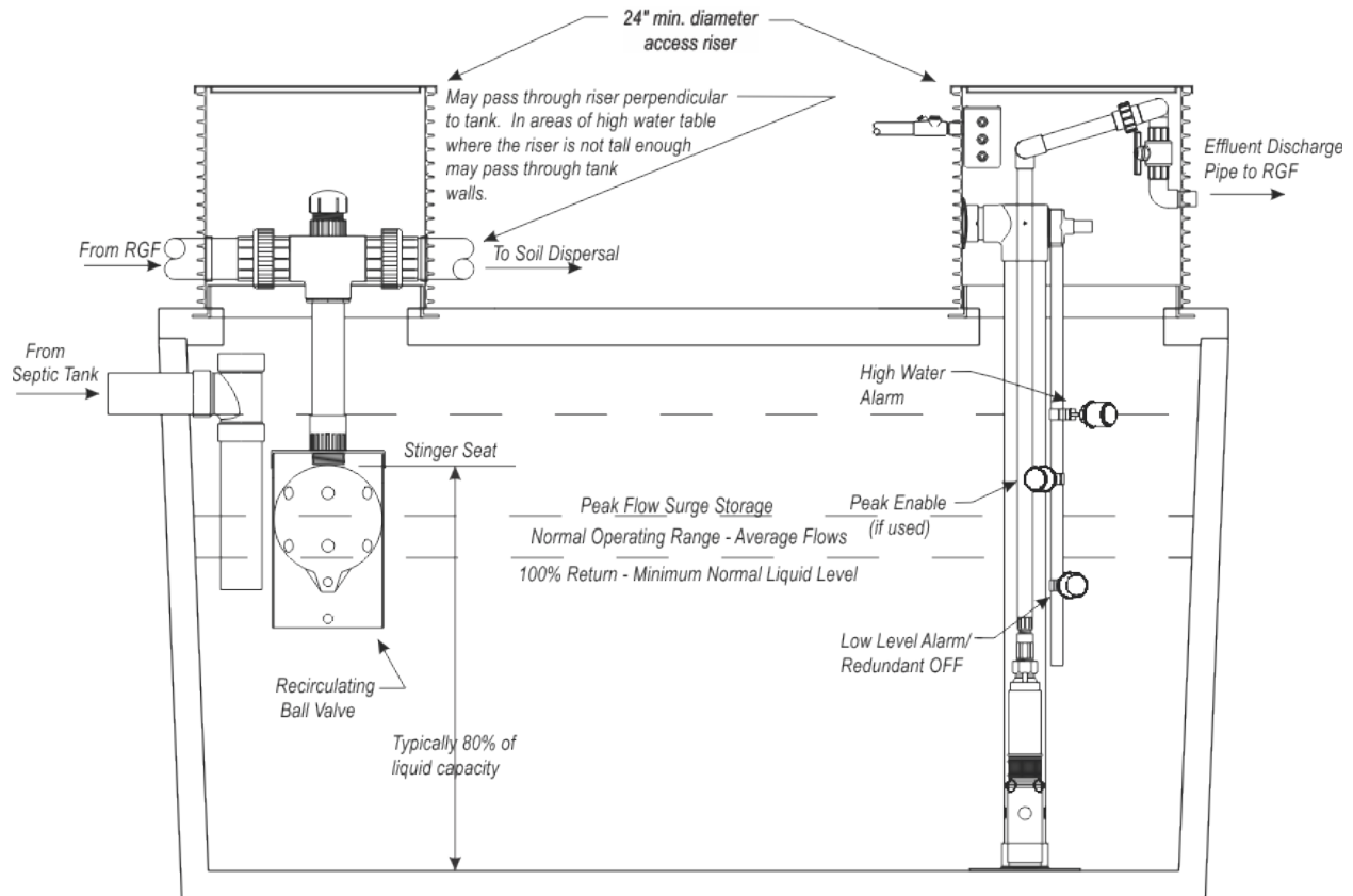
Figure 3. Example of a Recirculating/Mixing Tank with a Recirculating Ball Valve
