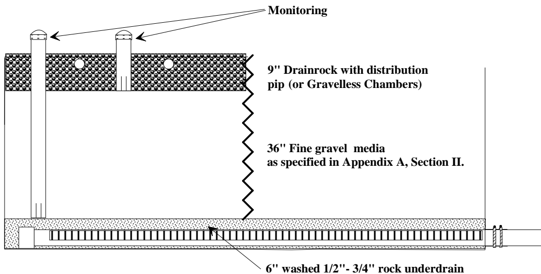
Figure 2. Cross-section of a Typical Recirculating Gravel Filter
