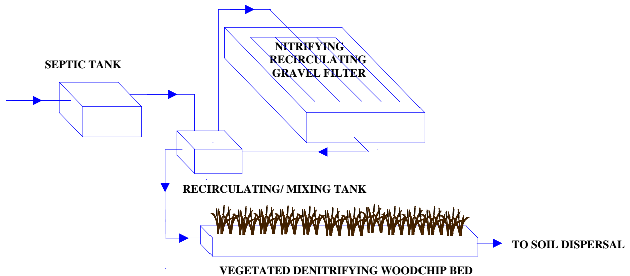
Figure 4. Layout of a Nitrifying Recirculating Gravel Filter and a Vegetated Denitrifying Woodchip Bed
