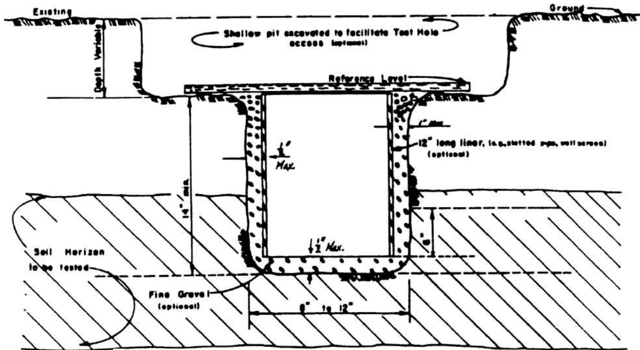
Figure 7. Percolation Test
