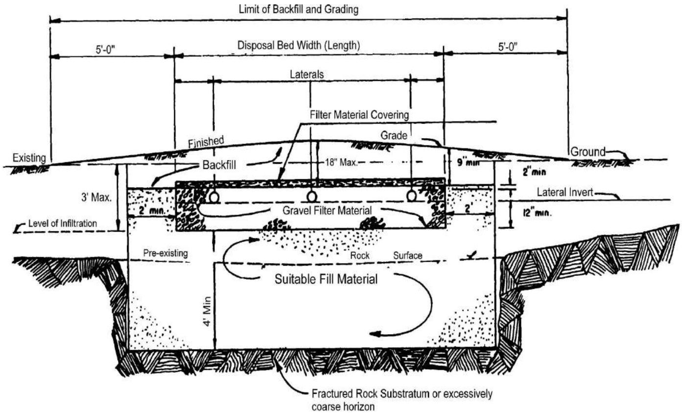
Figure 19. Soil Replacement, Fill-enclosed Disposal Field Installation
