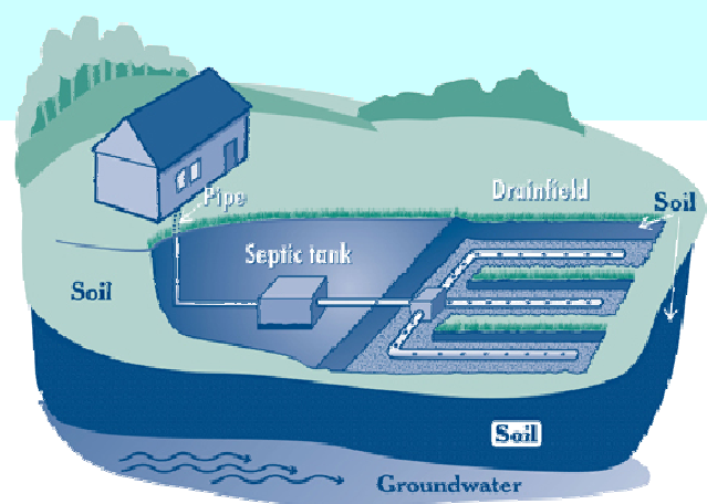
Typical onsite wastewater treatment system
