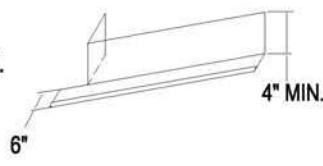
PAN OR CHANNEL FLASHING
