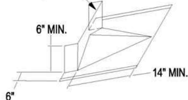
CRICKET FLASHING
