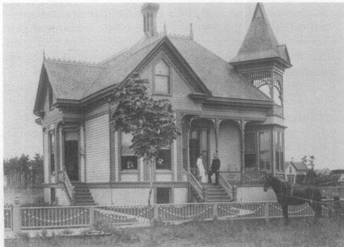
3. Readily available and inexpensive sawn shingles were used not only for roofs, but also for gables and wall surfaces. The circa 1891 Chambers House, Eugene, Oregon used straight sawn butts for the majority of the roof and hexagonal butts for the lower portion of the corner tower. Decorative shingles in the gable ends and an attractive wooden roof cresting feature were also used. Photo: Lane County Historical Society.
