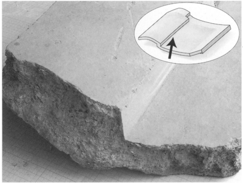
Figure 5. Break face across the cover-pan joint revealing the continuous fabric: Corinth FP 342. P. Sapirstein
