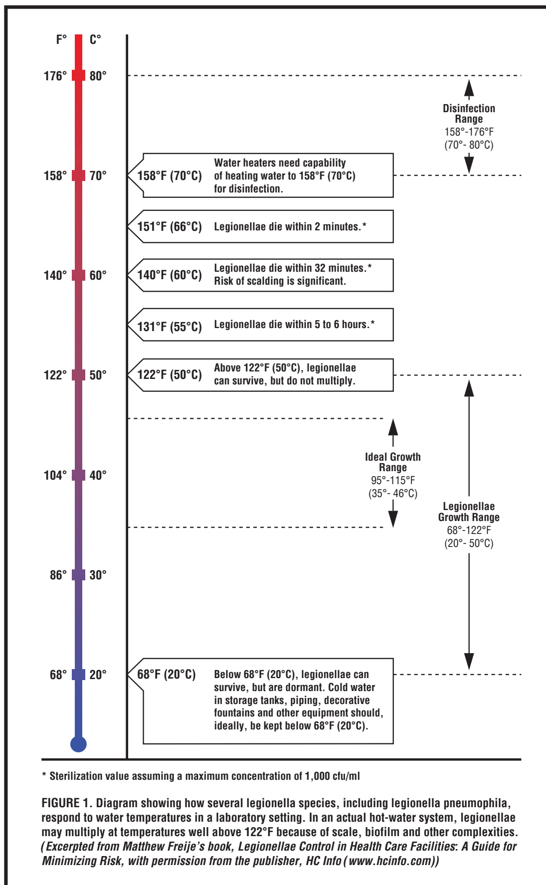
Figure 1 – Water Temperature Effects on Legionellae Bacteria
