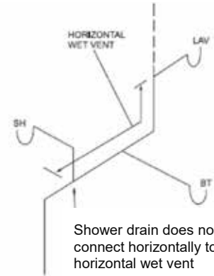
Noncompliant Horizontal Wet Vent
