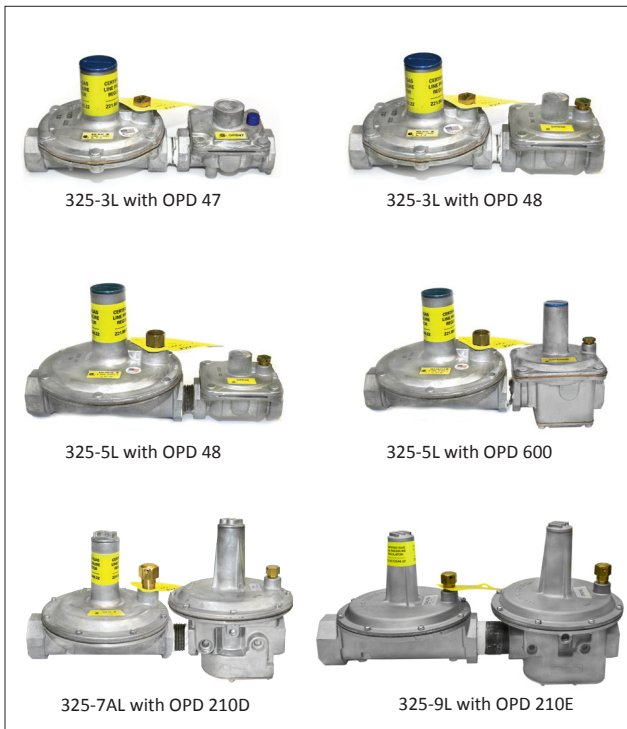
Figure 4: 325-L Models with OPDs
