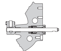
Stem Packing
