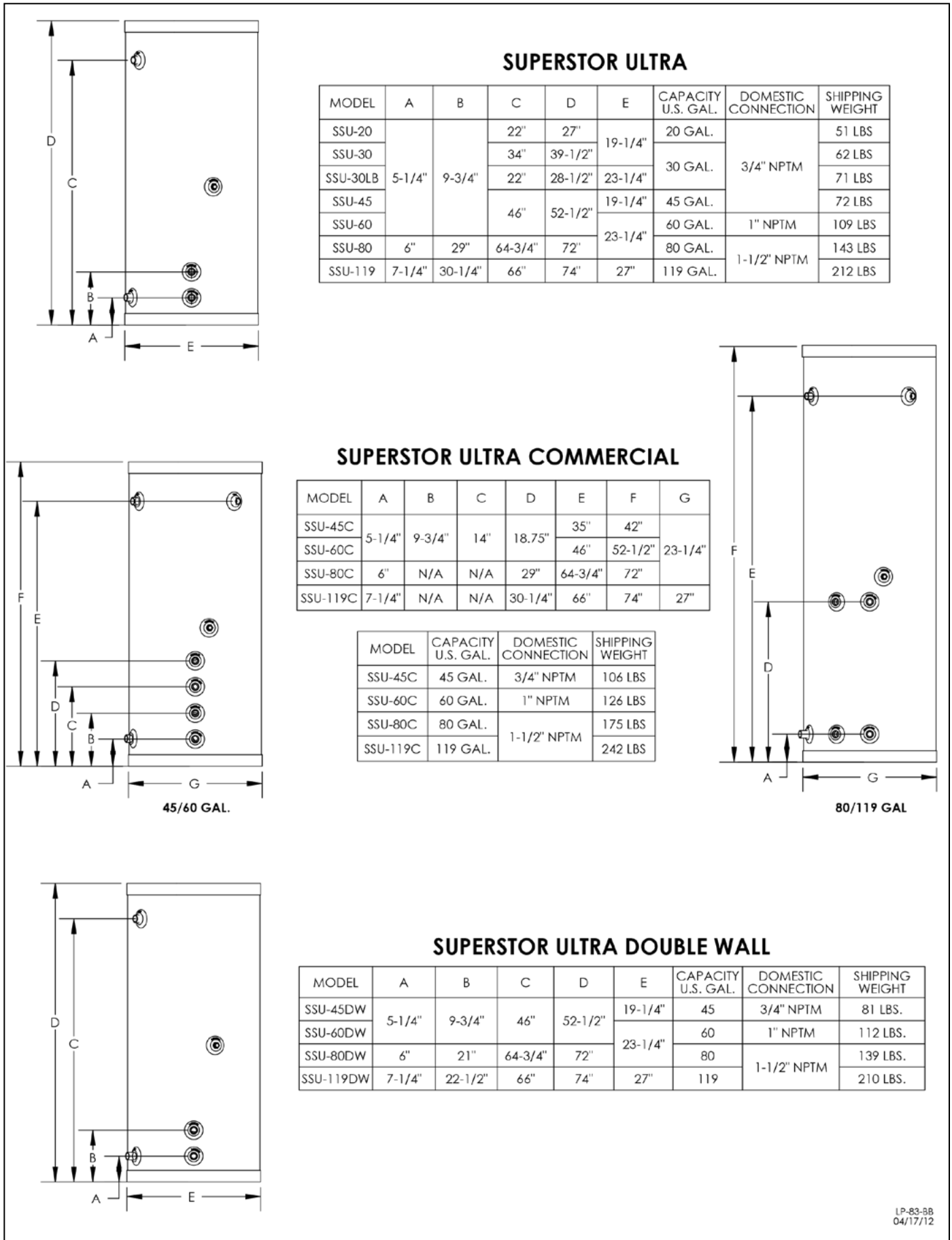
Figure 2 - Dimensions
