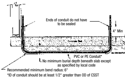
Figure 4.26 Installation in Nonmetallic Conduit Under Slab
