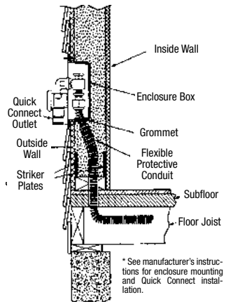
Figure 4.19 Quick Connect Outlet
