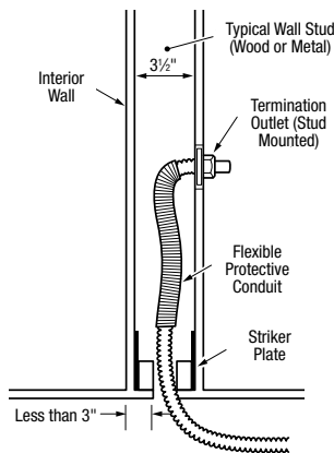
Figure 4.11 Use of Flexible Protective Conduit
