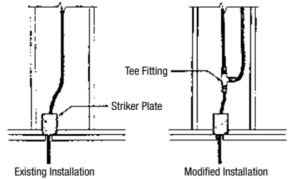
Figure 4.8 Extension of Existing Tubing Run
