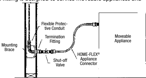
Figure 4.16 HOME-FLEX® Connection to Moveable Gas Appliance
