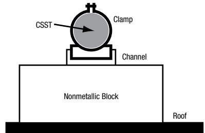
Figure 4.18 Rooftop Support with Strut
