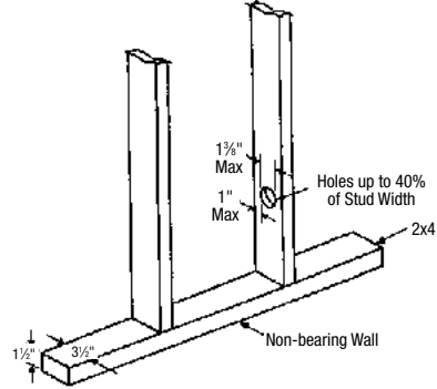
Figure 4.6 Holes in Bearing Walls
