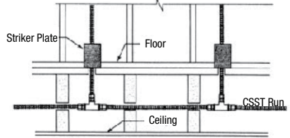
Figure 4.7 Multiple Outlets Along Main CSST Run
