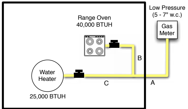
Figure 3.5 Low Pressure System—Series Arrangement
