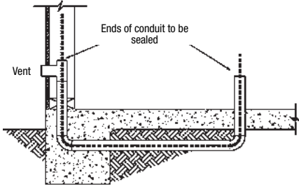
Figure 4.28 Installation in Nonmetallic Conduit with Venting
