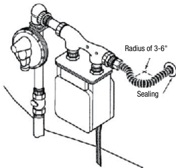
Figure 4.14 Independently Supported Meter
