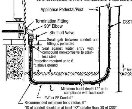
Figure 4.20 Fixed Outdoor Appliance (Underground Routing)
