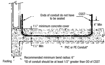
Figure 4.27 Installation in Nonmetallic Conduit In Slab
