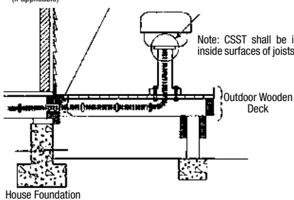
Figure 4.21 Fixed Outdoor Appliance (Deck Mounted)
