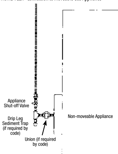
Figure 4.15 Direct Connection to Fixed Appliance
