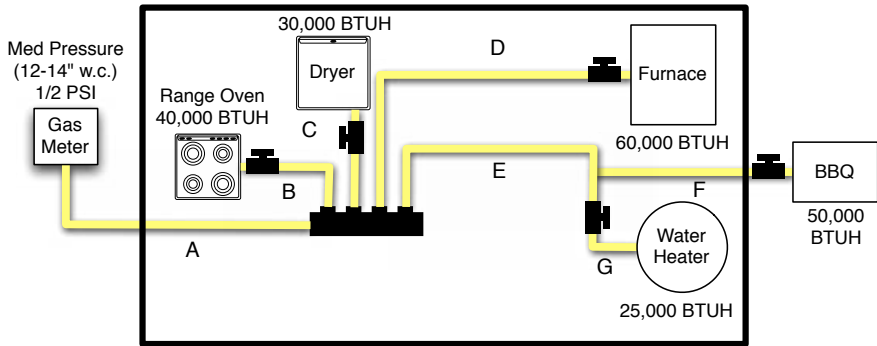
Figure 3.8 Medium Pressure System—Parallel Arrangement with Series Branch
