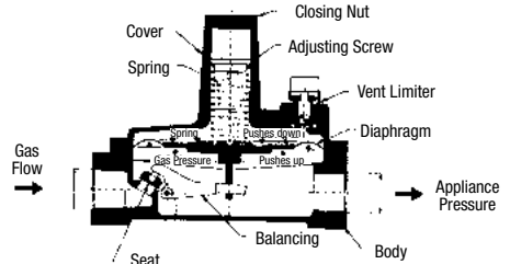
Figure 4.25 Pressure Regulator Diagram
