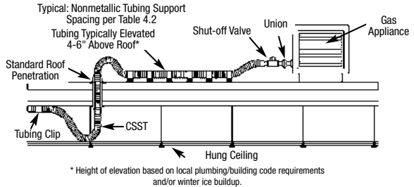
Figure 4.17 Roof Top Equipment Installation
