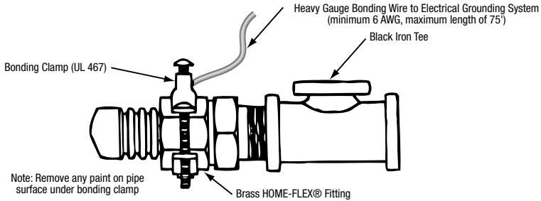
Figure 4.29 Bonding Connection to Brass Fitting
