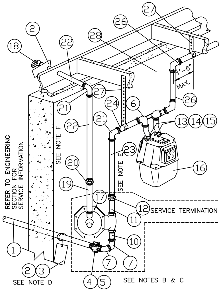
FOR HIGH PRESSURE SERVICE
