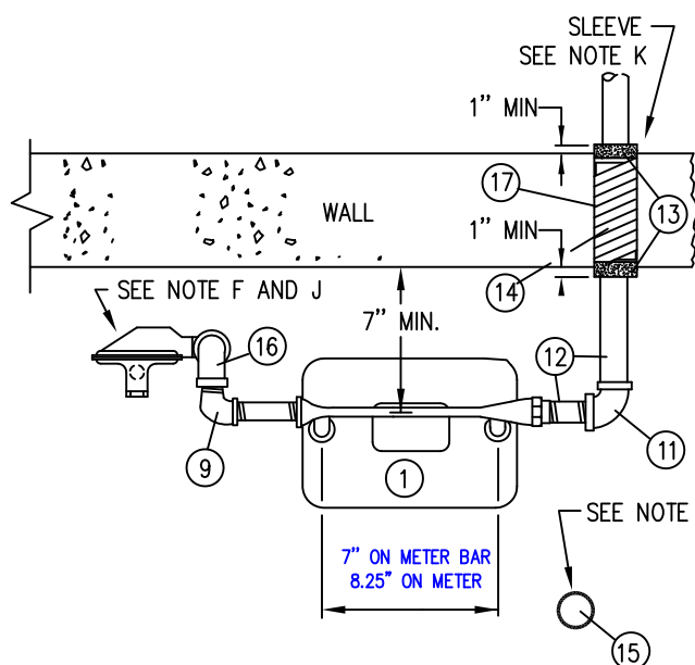
PLAN 425 CFH AND 630 TYPE
