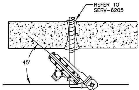
PLAN VIEW AT REGULATOR
