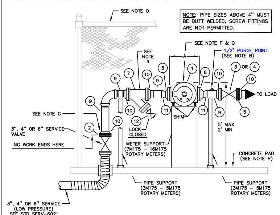
FRONT ELEVATION FIG. 3 - OUTSIDE SET 3", 4" OR 6" SERVICE
