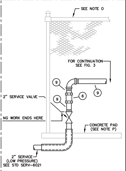
FRONT ELEVATION FIG. 4 - OUTSIDE SET 2" SERVICE
