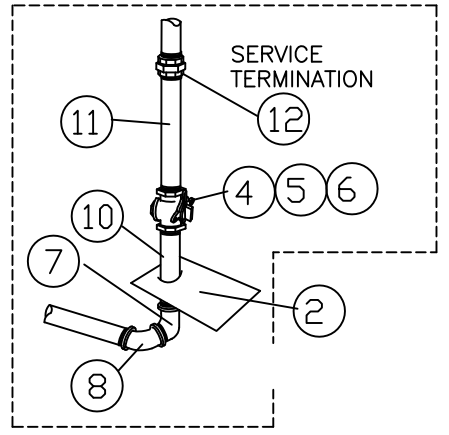
FOR LOW PRESSURE SERVICE
