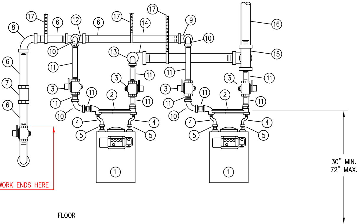
ELEVATION 250 CFH TYPE
