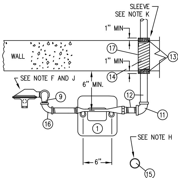
PLAN 250 CFH TYPE
