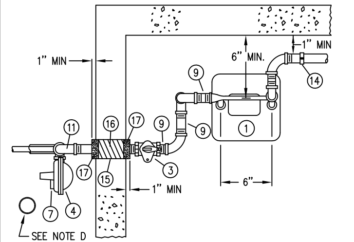
PLAN 250 CFH TYPE
