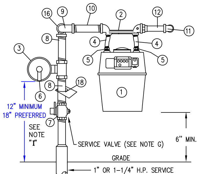
ELEVATION 425 CFH AND 630 TYPE
