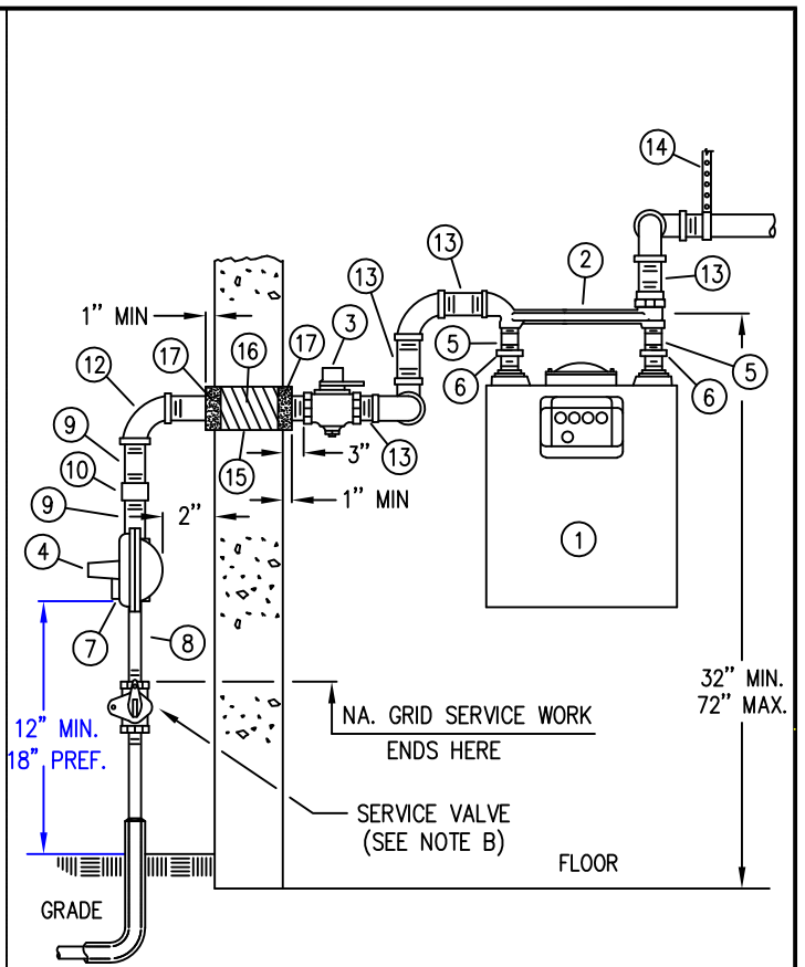
ELEVATION 425 CFH TYPE
