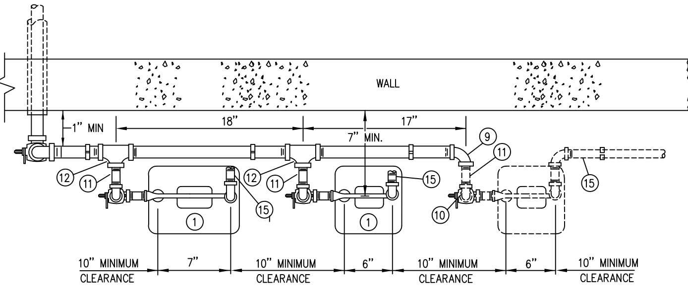
ELEVATION 250 CFH AND 425 CFH TYPE
