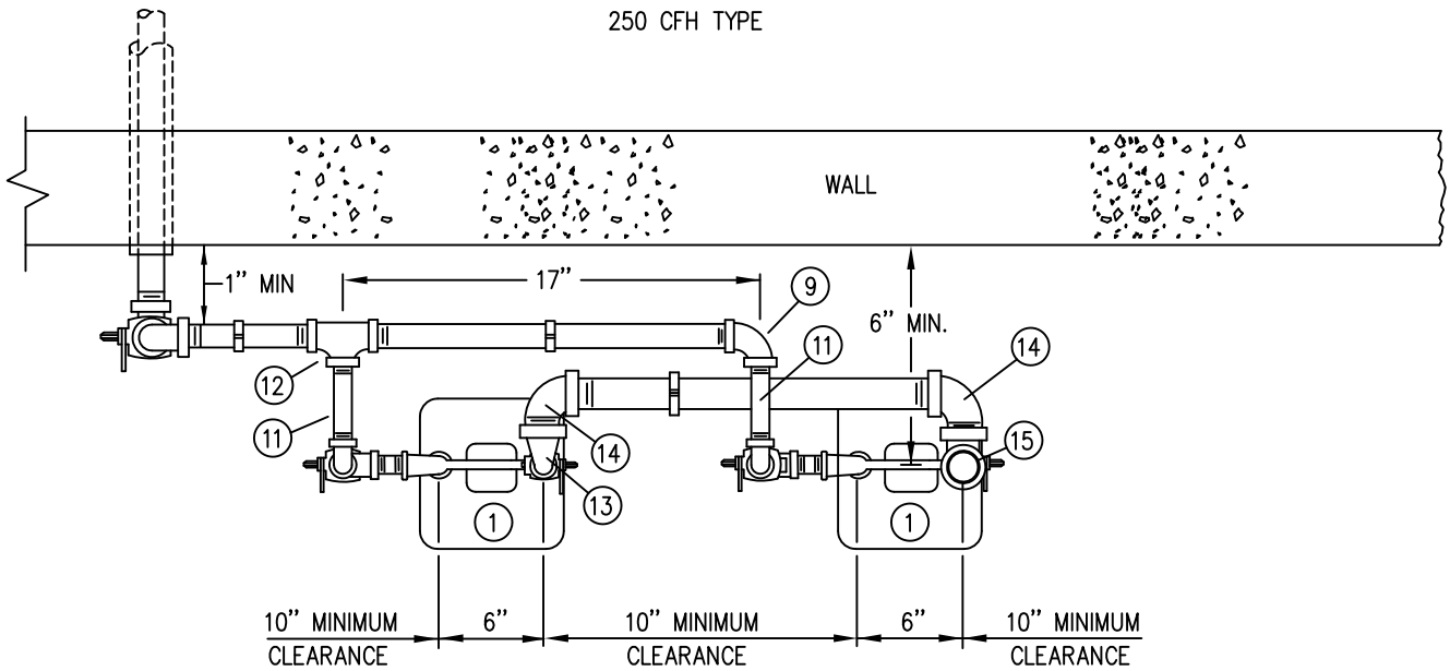
PLAN 250 CFH TYPE
