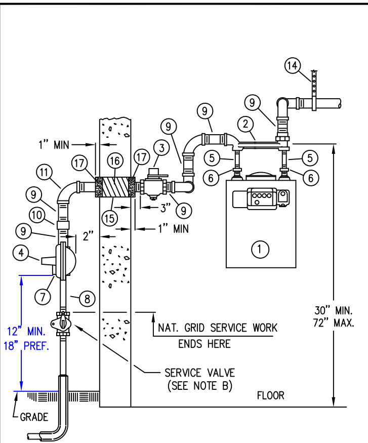
ELEVATION 250 CFH TYPE
