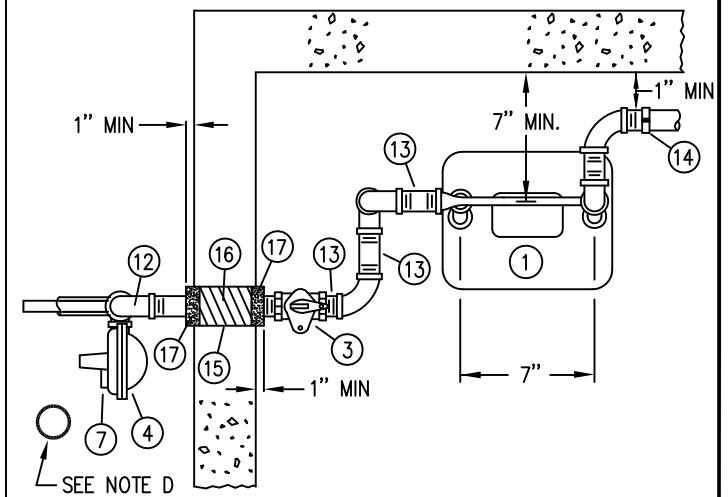
PLAN 425 CFH TYPE
