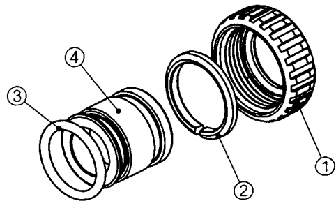
Order No: V3007-05 Description: WS1 Fitting 1-¼" Plastic Male Assembly
