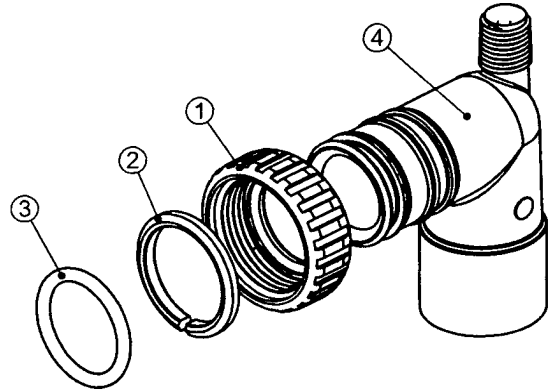
Order No: V3007-03 Description: WS1 Fitting ¾" Brass Sweat Assembly
