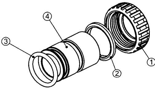
Order No: V3007-04 Description: WS1 Fitting 1" Plastic Male NPT Assembly
