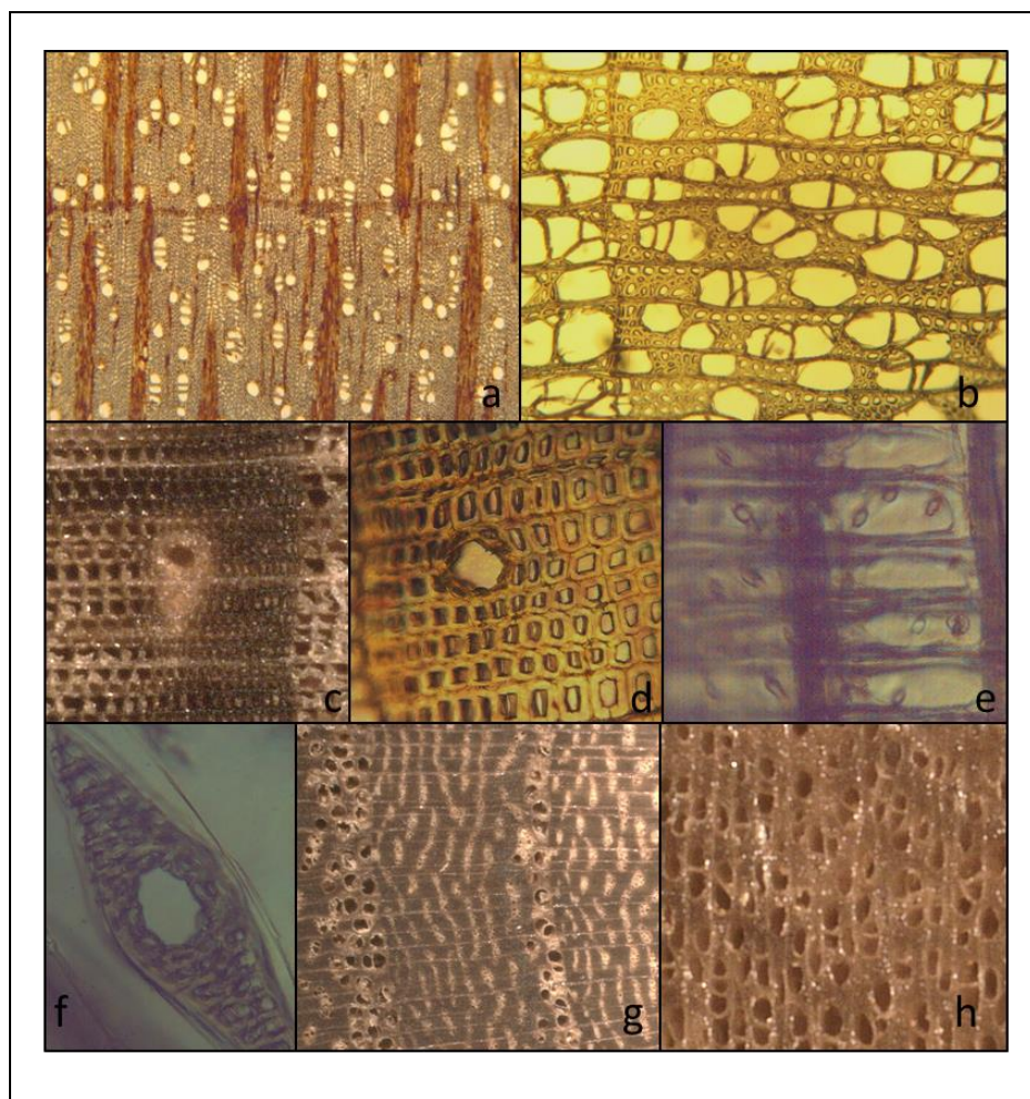
Figure 3. Anatomical features of the examined wood samples: (a) Maple: transversal section (microscopy magnification 40x); diffuse porous wood with a distinct growth ring and pluriserial rays up to 6 rows of parenchymatic cells. (b) Poplar: transversal section (10x); diffuse porous wood with a distinct growth ring and uniserial rays. (c, d) Spruce: softwood with resin canal, thin-walled epithelial cells (stereoscopy 32x, optic microscope 25x). (e) Spruce: radial section (40x); pits in cross-field small, 2-3 per cross-field. (f) Spruce: resin canal in tangential section (40x). (g) Elm: transversal section (12,5x); porous rings in early wood, latewood pores in wavy (ulmiform) tangential bands. (h) Poplar: transversal section (11x); diffuse porous with uniserial rays.
