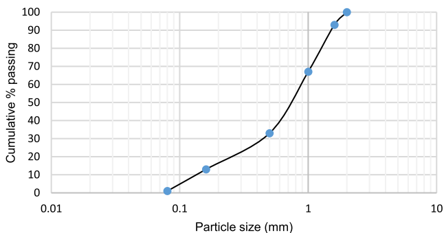
Fig. 1. Particle size distribution for standard sand.
