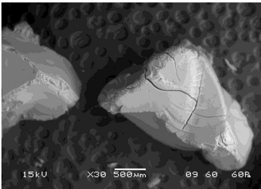
Fig. 6. Aerogel particles as manufactured.
