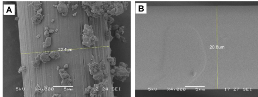
Fig. 8. Fibre extracted from fracture surface of test specimen (image A). Fibre in as-manufactured condition (image B).
