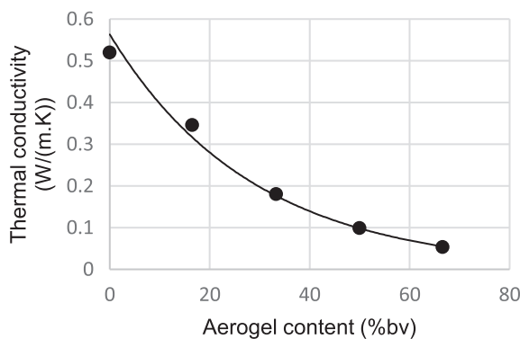
Fig. 12. Effect of aerogel content on thermal conductivity.
