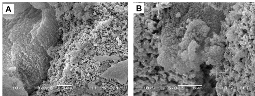
Fig. 9. Calcite crystals adhering to aerogel particles (image A). Aerogel particle entrapped within calcite (Image B).
