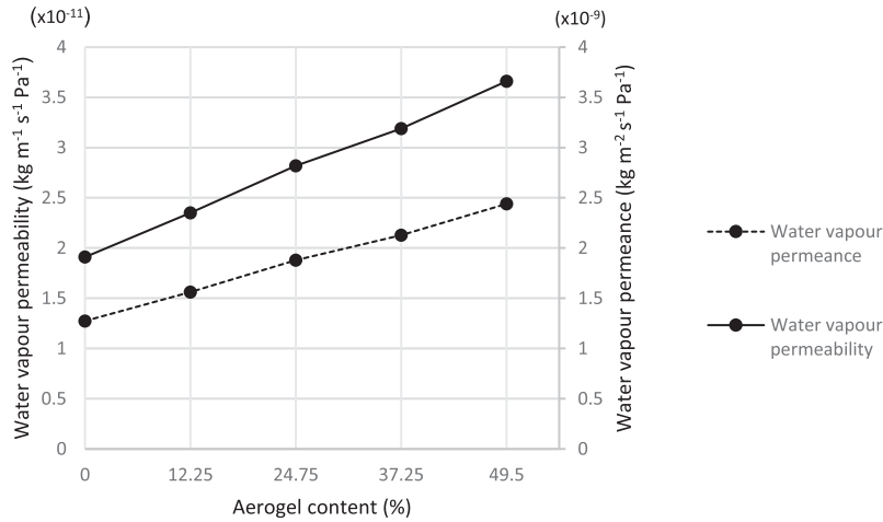
Fig. 14. Aerogel effect on water vapour permeability.
