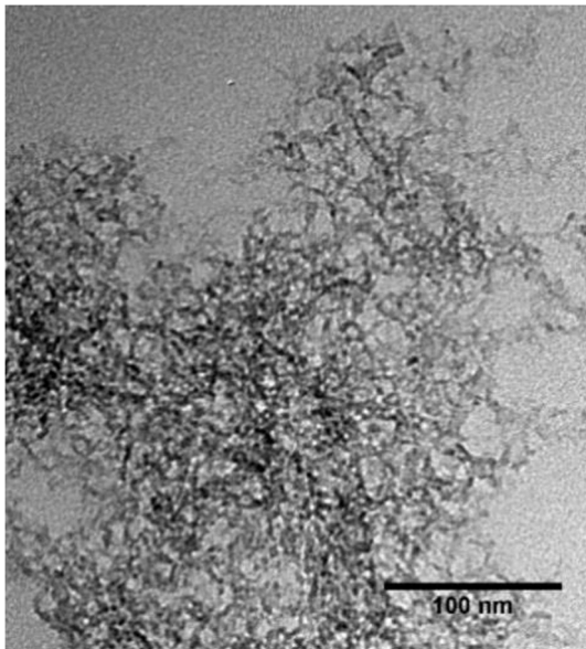
Fig. 11. TEM image of a crushed aerogel particle showing the highly porous nature of its internal structure. (Magnification = 250,000 \times ).
