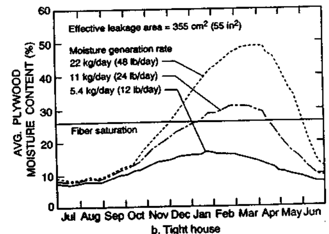
Figure 5 Effect of moisture generation rate in Madison, Wis.
