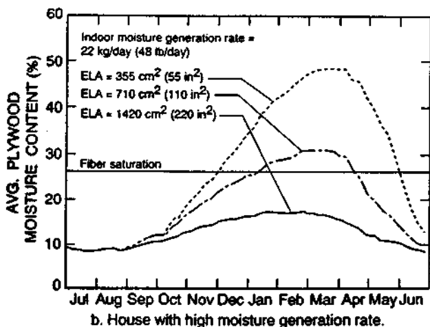
Figure 4 Effect of effective leakage area (ELA) in Madison, Wis.
