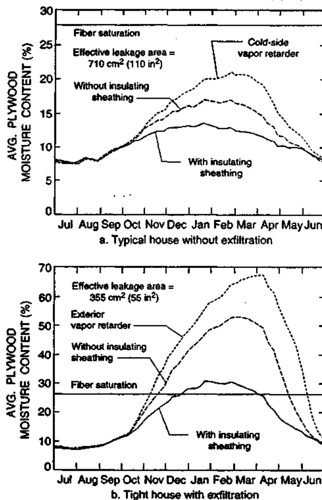
Figure 7 Effect of exterior insulating sheathing and exterior vapor retarder in Madison, Wis.
