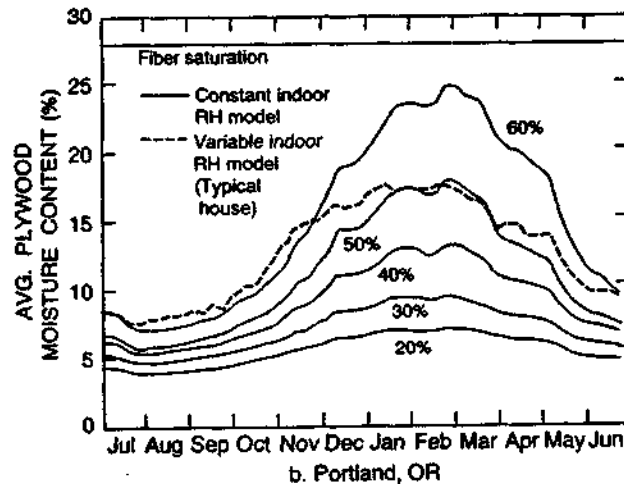
Figure 2 Comparison of constant and variable indoor RH model results.
