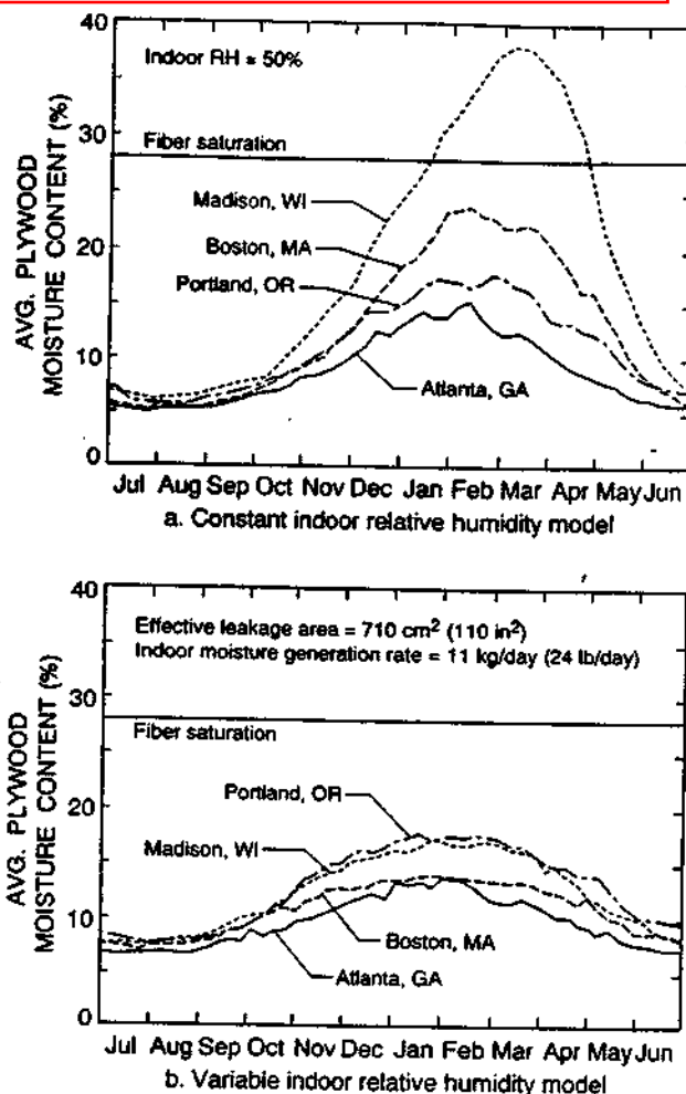
Figure 1 Effect of climate on plywood moisture content.
