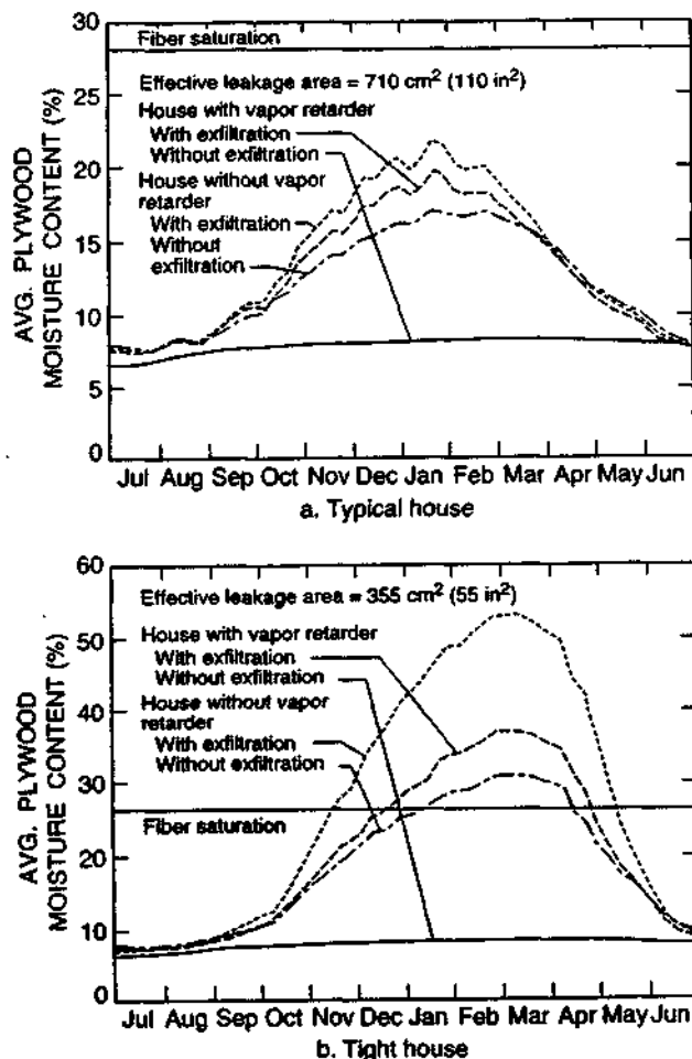
Figure 6 Effect of exfiltration on houses with and without an interior vapor retarder in Madison, Wis.
