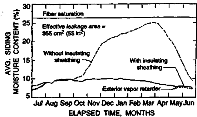
Figure 8 Effect of exterior insulating sheathing on wood siding moisture content for a tight house with exfiltration in Madison, Wis.
