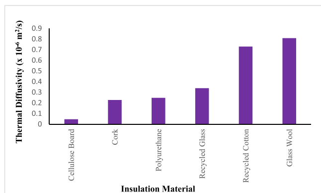
Fig. 2. Mean thermal diffusivity of various insulation materials.
