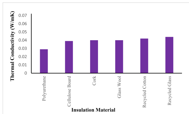
Fig. 1. Mean thermal conductivity of various insulation materials.
