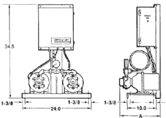
Dimensions Duplex Manual
