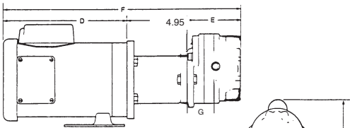
SPMV SINGLE SUPPLY UNIT
