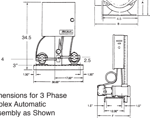
SPMV DUPLEX AUTOMATIC SUPPLY UNIT
