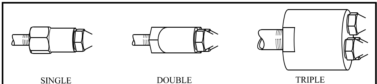
NOZZLE ARRANGEMENTS
