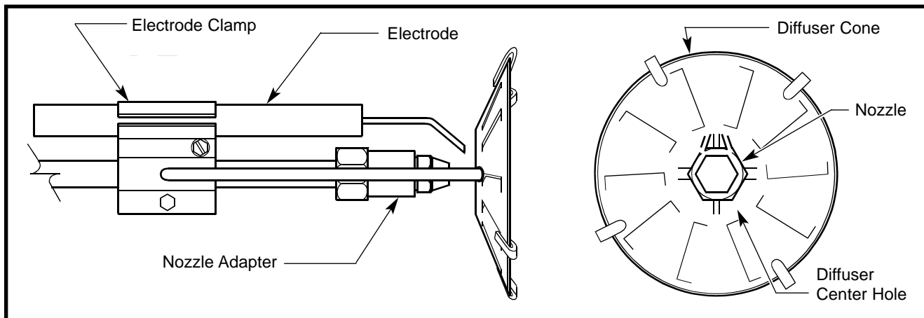
TYPICAL AIR DIFFUSER, NOZZLE AND ELECTRODE ARRANGEMENT
