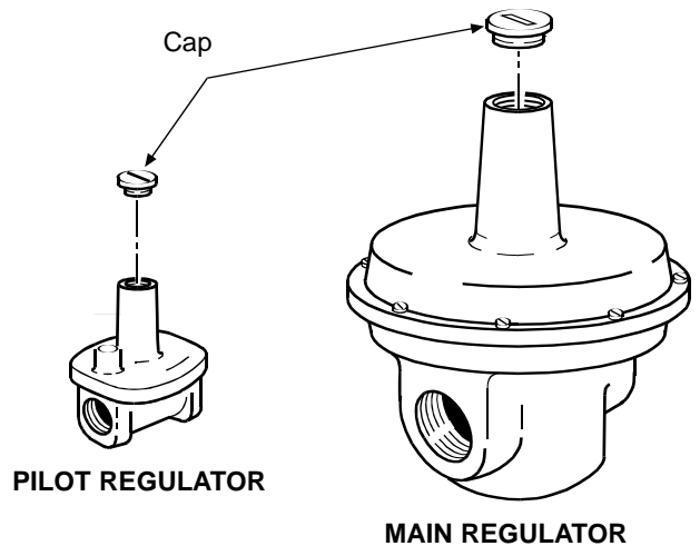
MAIN REGULATOR
