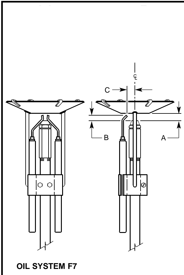
SINGLE VARIFLOW
