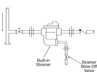
Fig. 3-4. No. 880-883 with strainer blow-down valve.
