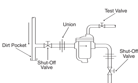
Fig. 3-1. Standard hookup No. 800-816, 800-883 traps, with shut-off valves to isolate trap during testing, inspection or repair. Unions should be at right angles—not in-line—to facilitate trap removal.
