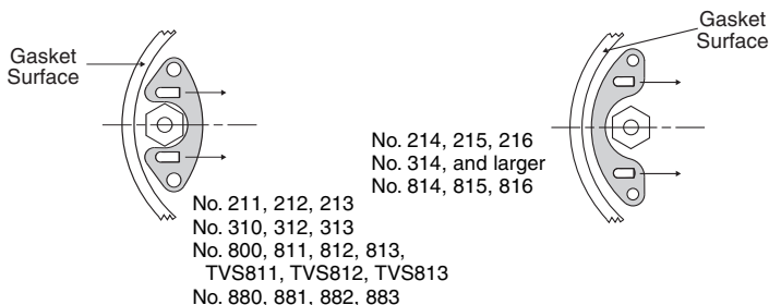
Fig. 12-6. Guide Pin Plate Locations. Pins always point away from adjoining Gasket Surfaces.
