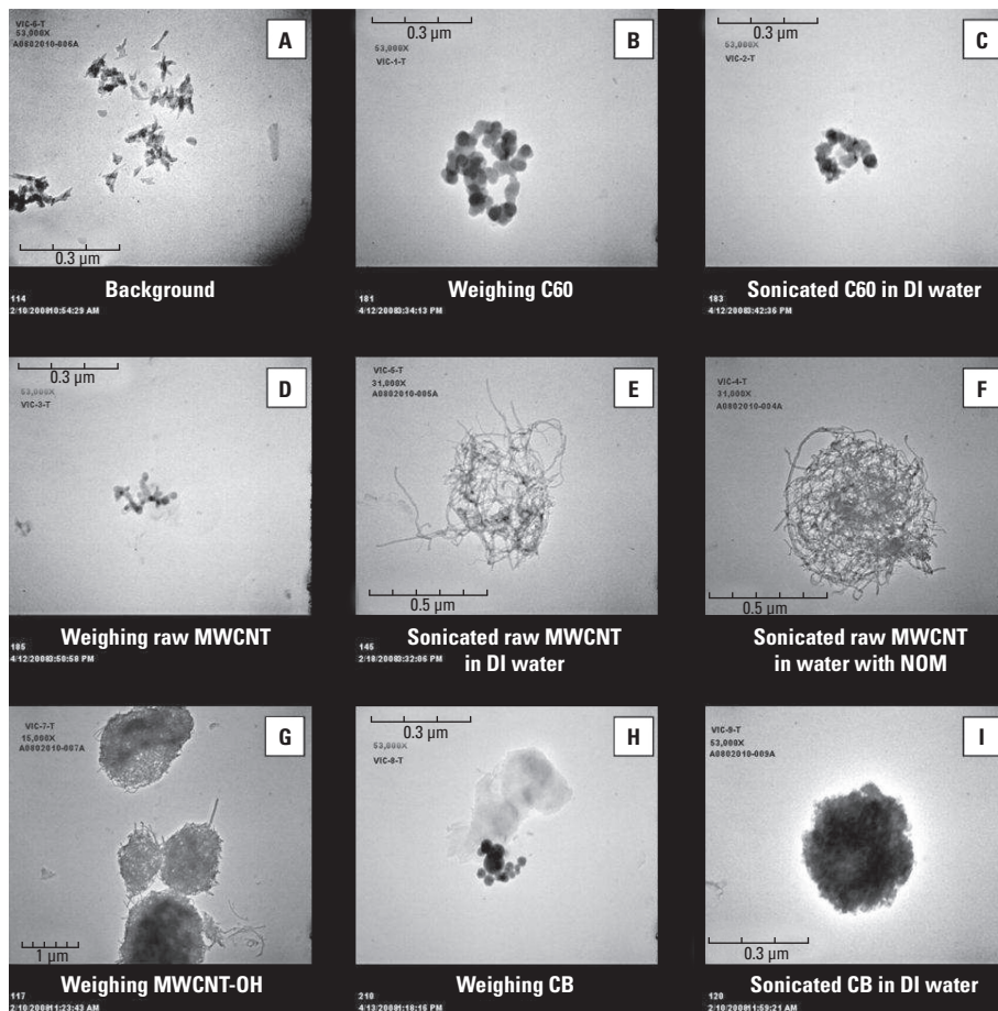
Figure 3. TEM images of engineered CNMs during laboratory processes. (A) Background air sample; bar = 0.3 \mu\text{m} . (B) Weighing/transferring C60 inside hood with no ventilation; bar = 0.3 \mu\text{m} . (C) Sonicating C60 in DI water inside unventilated enclosure; bar = 0.3 \mu\text{m} . (D) Weighing/transferring raw MWCNT inside hood with no ventilation; bar = 0.3 \mu\text{m} . Note that no tubular structures are present. (E) Sonicating raw MWCNT in DI water inside unventilated enclosure; bar = 0.5 \mu\text{m} . (F) Sonicating raw MWCNT in reconstituted water containing 100 mg/L (parts per million) NOM inside unventilated enclosure; bar = 0.5 \mu\text{m} . (G) Weighing/transferring MWCNT-OH inside hood with no ventilation; bar = 1 \mu\text{m} . (H) Weighing/transferring CB inside hood with no ventilation; bar = 0.3 \mu\text{m} . (I) Sonicating CB in DI water inside unventilated enclosure; bar = 0.3 \mu\text{m} .
