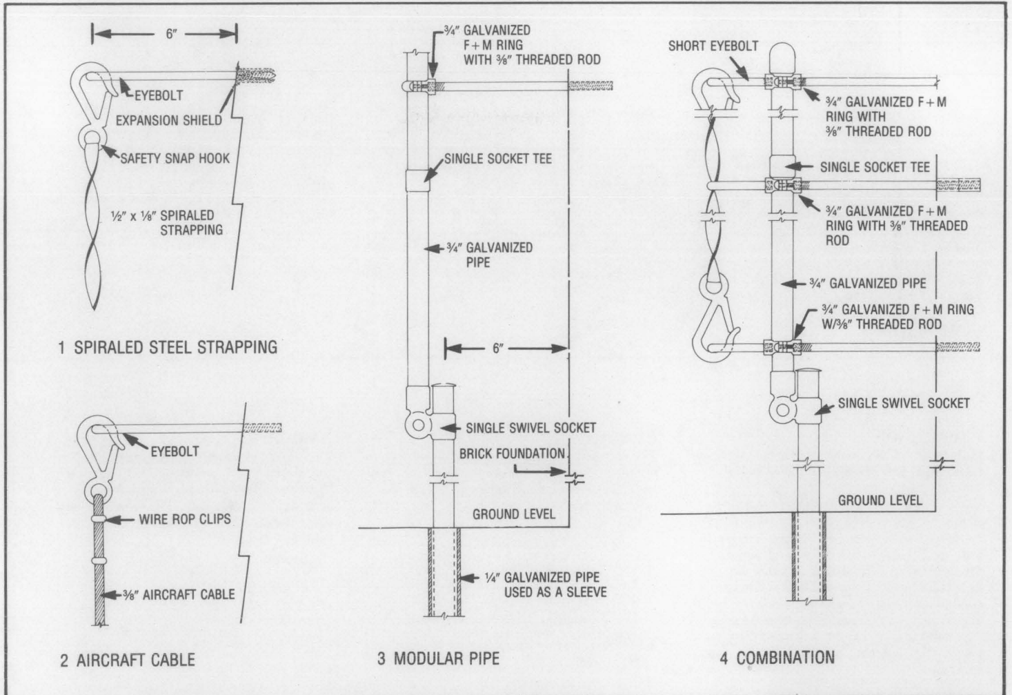
Figure 5. Details of the four experimental trellis systems. Drawings by Sharon Runner, National Park Service.
