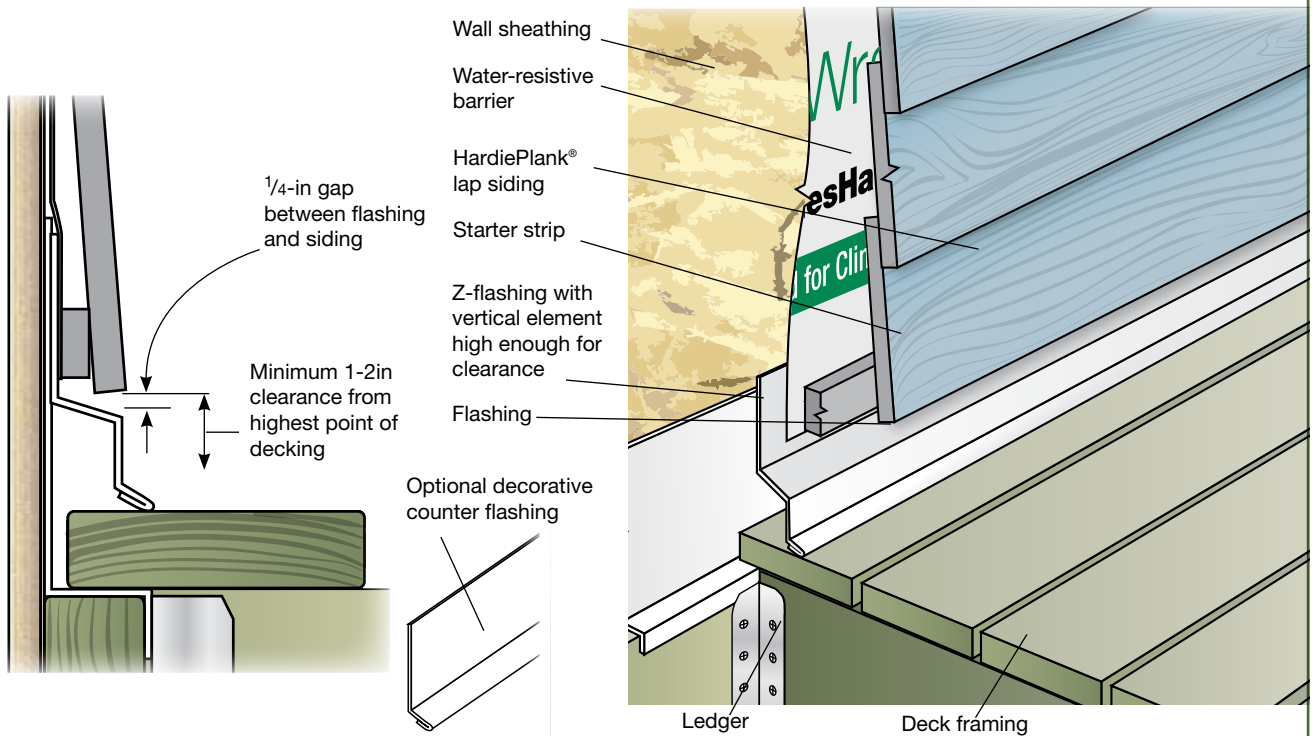
4.38 Wall to deck intersection with decorative counter flashing
