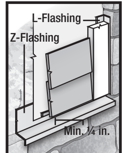
Figure 11 Mortar/Masonry
