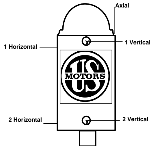
Figure 2: Vertical Motors (front view of motor)
