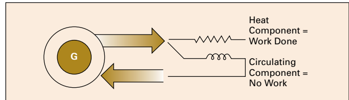
Figure 3. kVA Power
