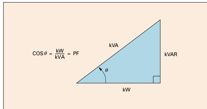
Figure 4. Power Triangle
