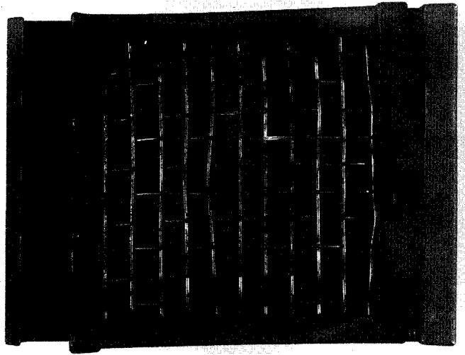
FIGURE 5-4. STEEL MESH TO HOLD INSULATION FROM LARGE GAUGE WIRE IN PLACE
