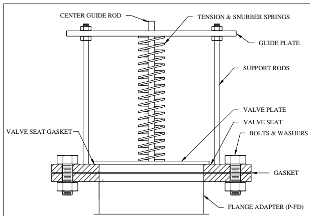
Fig. F-10 - Excessive Pressure Relief Valve (P-ER)
