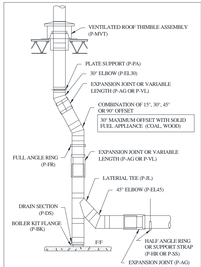
Fig. B-6 - Base Supported Stack with Offset
