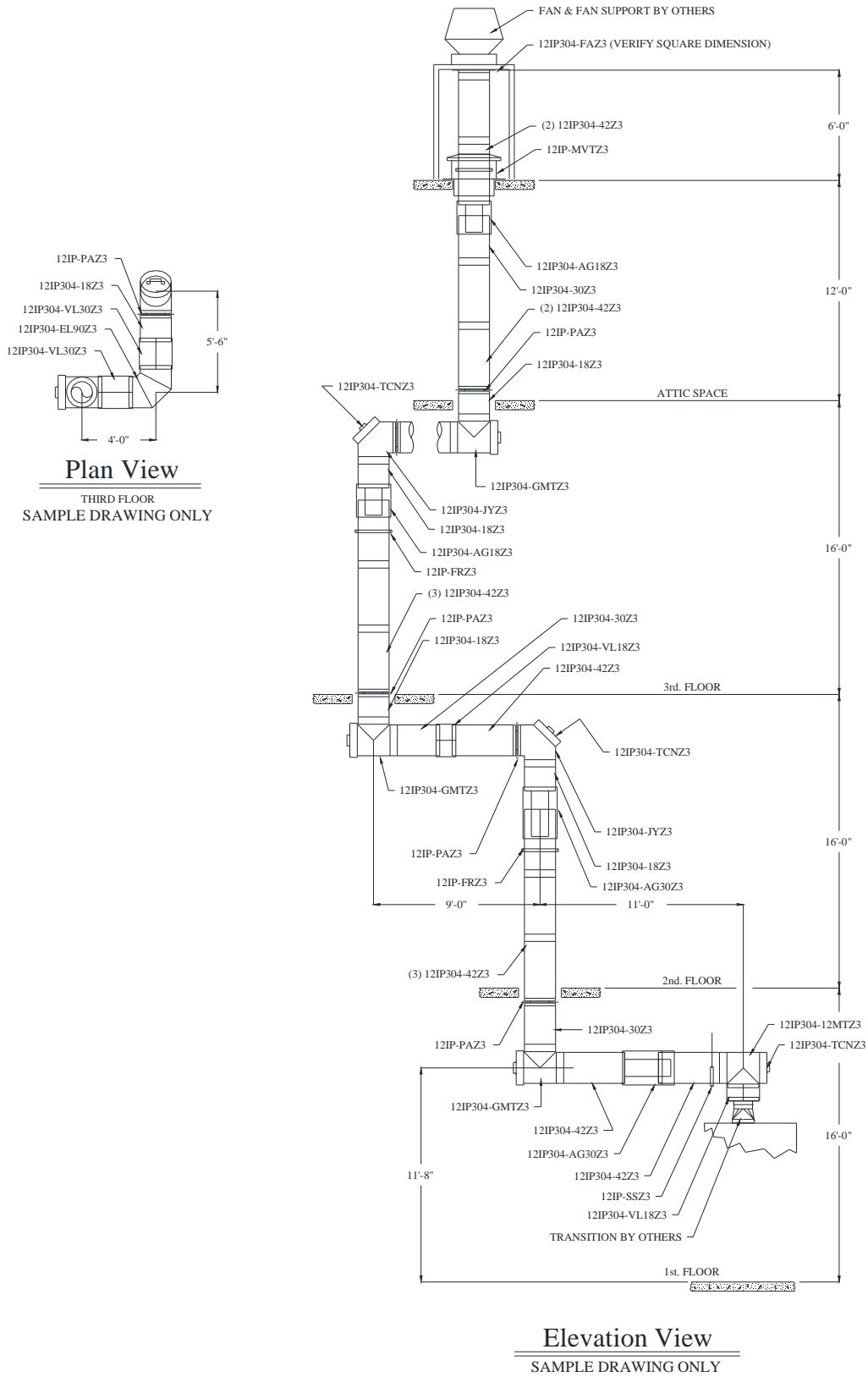
Fig. G-21 Sample Drawing (Grease Duct Installation)
