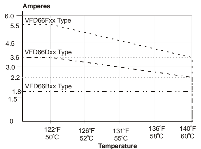
Figure 11: 400/460 VAC Temperature De-Rating
