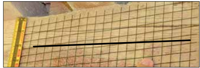
Figure 6.9—Use of grid to easily estimate the slope of grain. The 2:18 grids above implies 1 in 9 slope of grain. The black line shows the direction of slope of grain.
