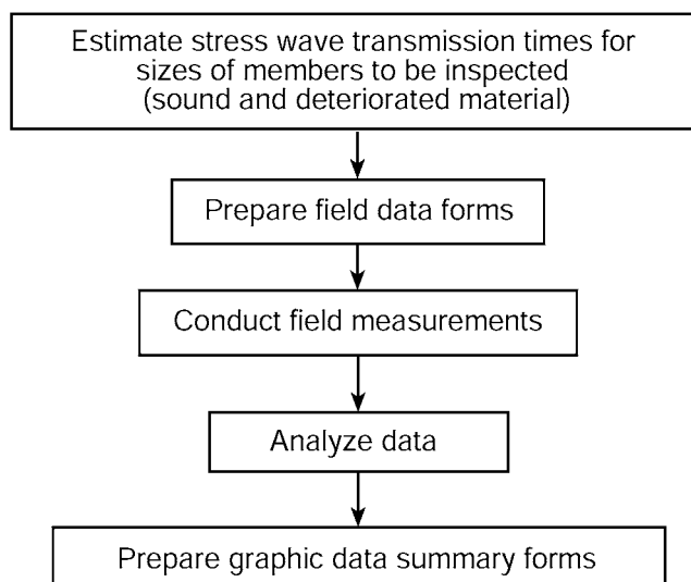
Figure 3.10—General procedures used to prepare and use stress wave timing methods for field work.
