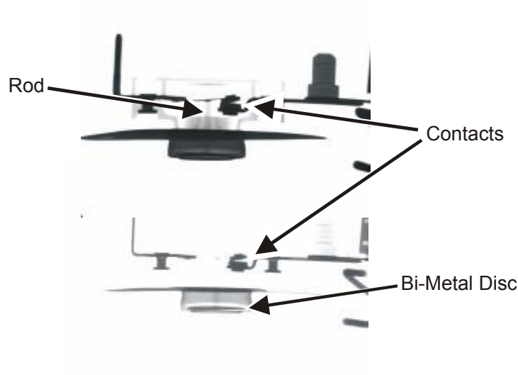
Figure 106. X-ray Images of High-Limit Thermostat 2 (HLT2)
