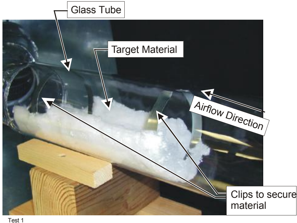
Figure 68. Setup with Target Material in the Glass Tube
