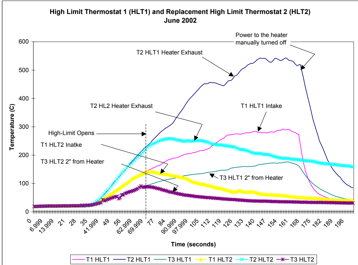
Figure 100. Failed Thermostat compared to a Replacement Thermostat
