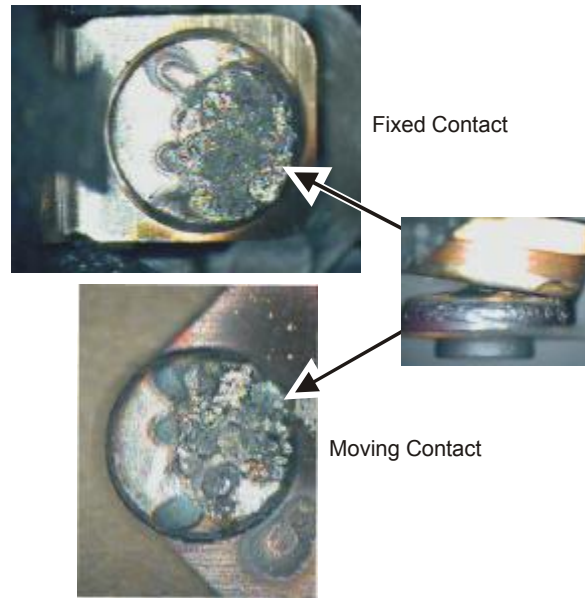
Figure 103. Contact Pads for High-Limit Thermostat 1 (HLT1)
