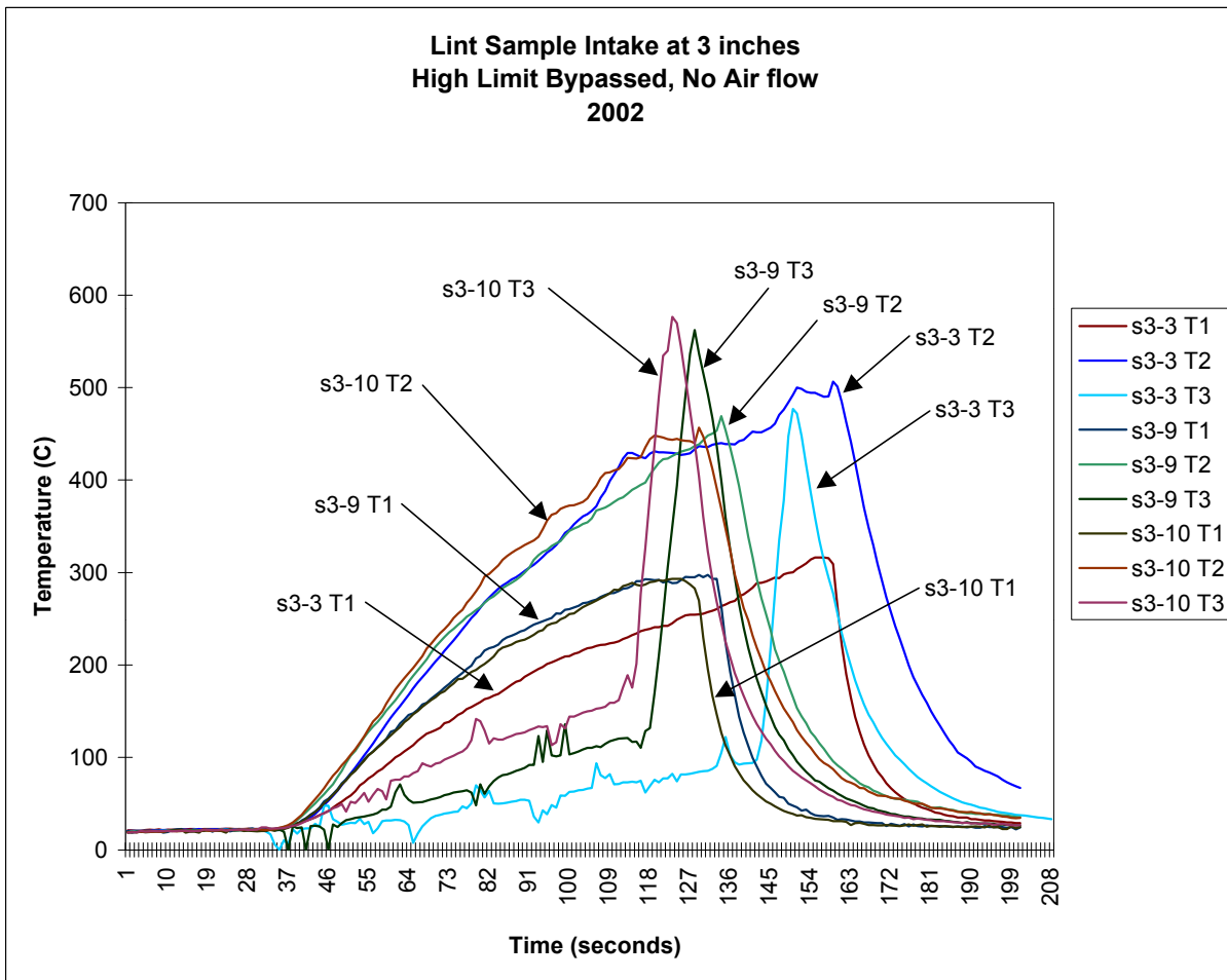
Figure 88. Lint Samples Tested 3 Inches from the Heater Housing Edge
