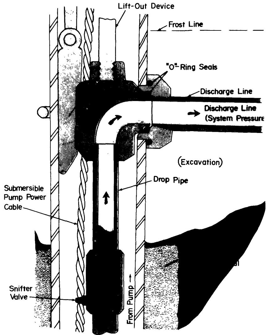
FIGURE 28. - Clamp-on pitless adapter for submersible pump installation
