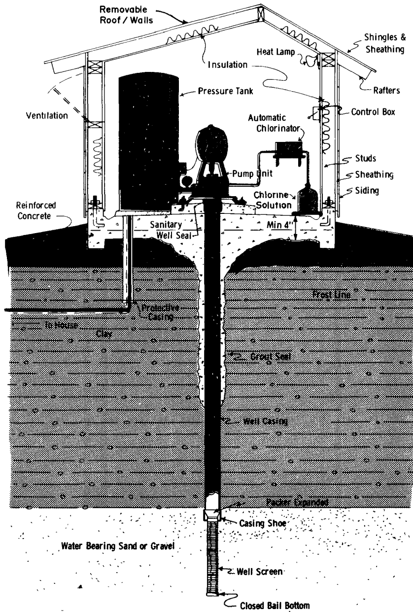
FIGURE 27. - Pumphouse.
