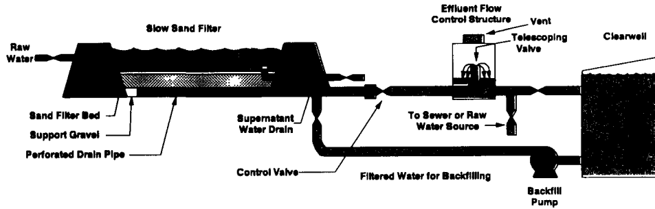
Typical unboxed slow sand filter installation
