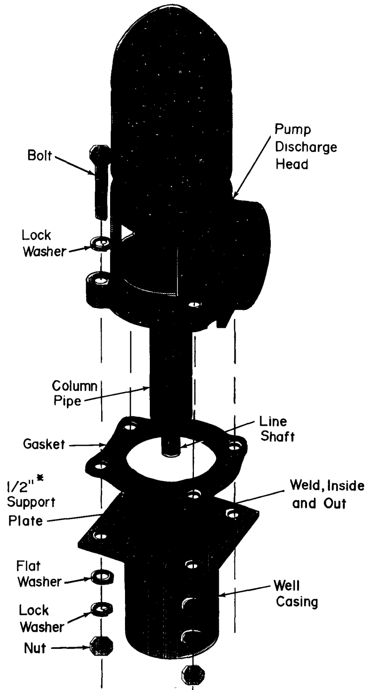
FIGURE 26. - Vertical (line shaft) turbine pump mounted on well case.
