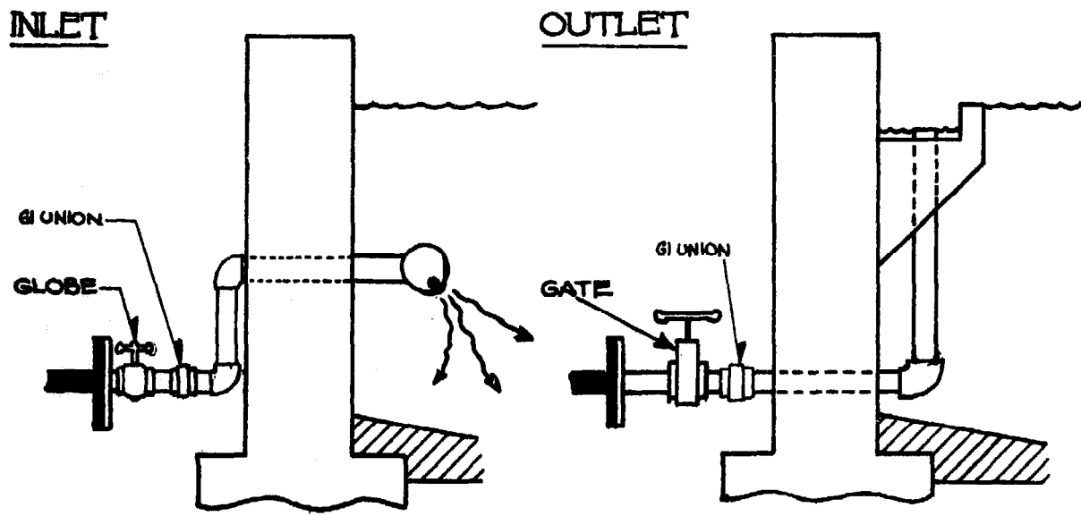
FIGURE 12-1 RECOMMENDED SEDIMENTATION TANK
