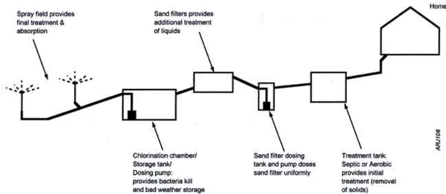
Figure 1. Components of an IRSIS on-lot sewage land application system.
