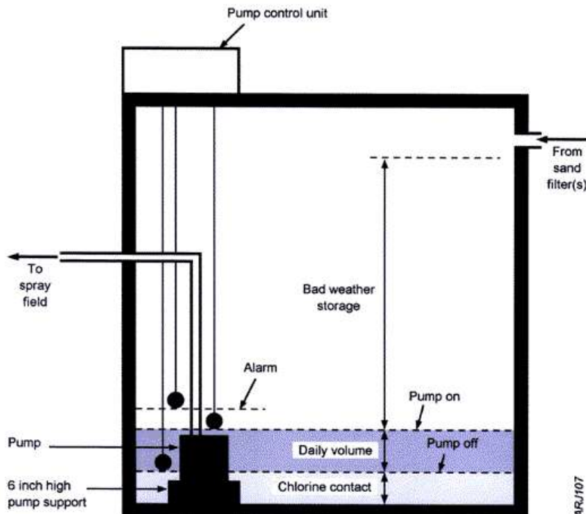
Figure 6. Chlorine contact and storage tank.
