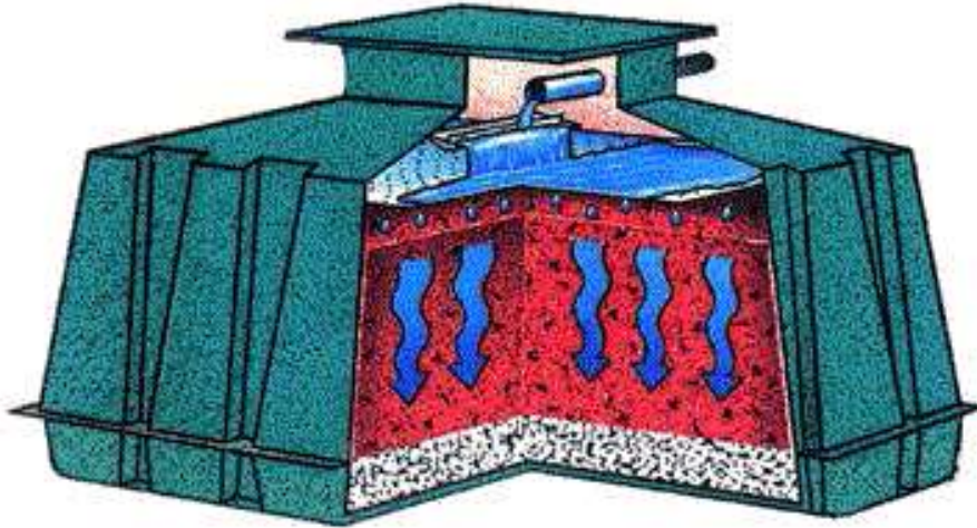
Figure 5. Peat Bio-filter.
