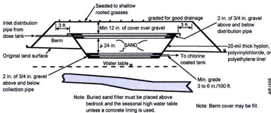
Figure 4. Buried sand filter.
