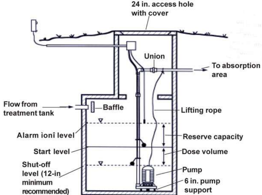
Figure 2. Typical dose tank and pump installation.
