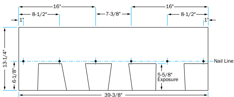
MANSARD AND HIGH WIND WARRANTY FASTENING PATTERN
