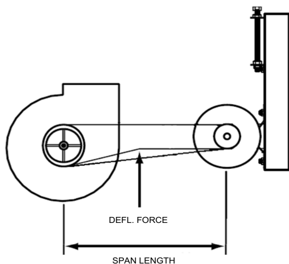
Figure 23: Belt Adjustment
