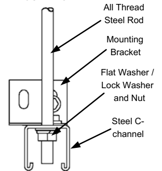
MOUNTING DETAIL
