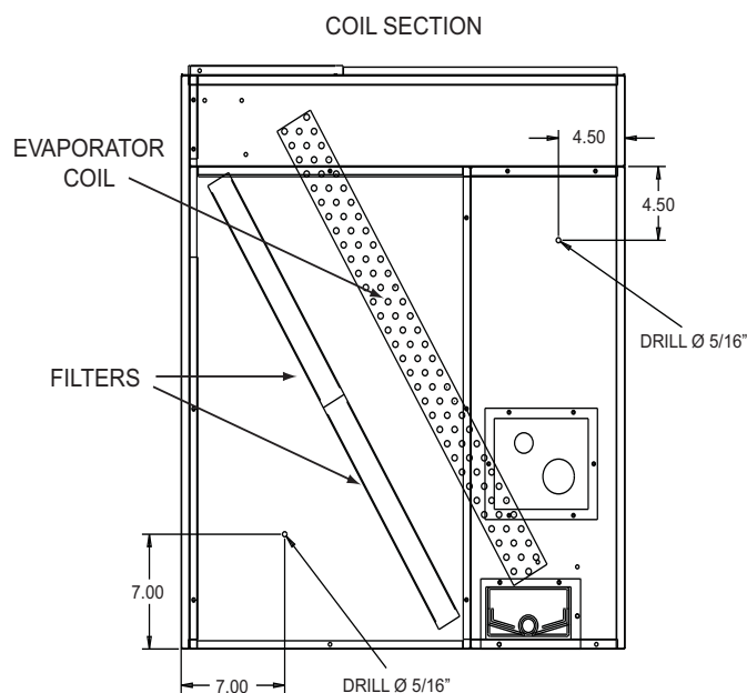
Figure 21: Hole Location For Pressure Drop Reading
