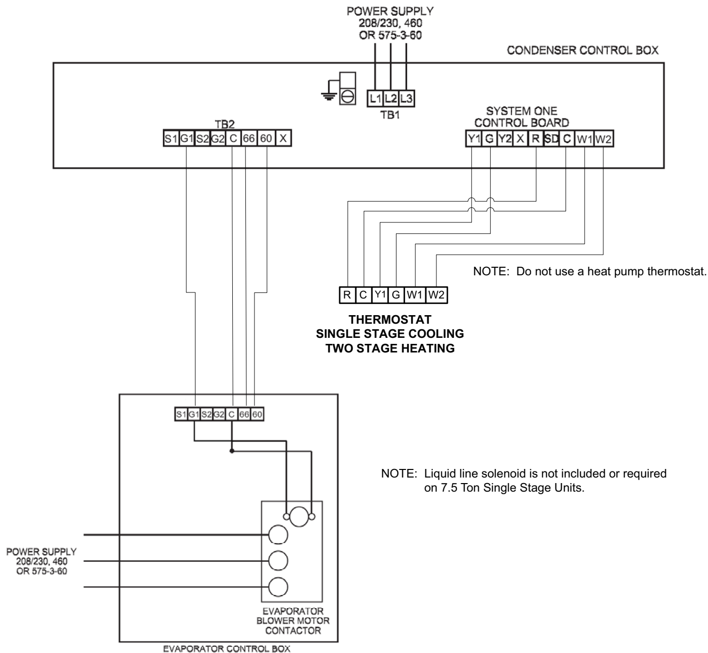
Figure 8: Typical Field Wiring Diagram - NH-07 Evaporator Unit with PH-07 Heat Pump
