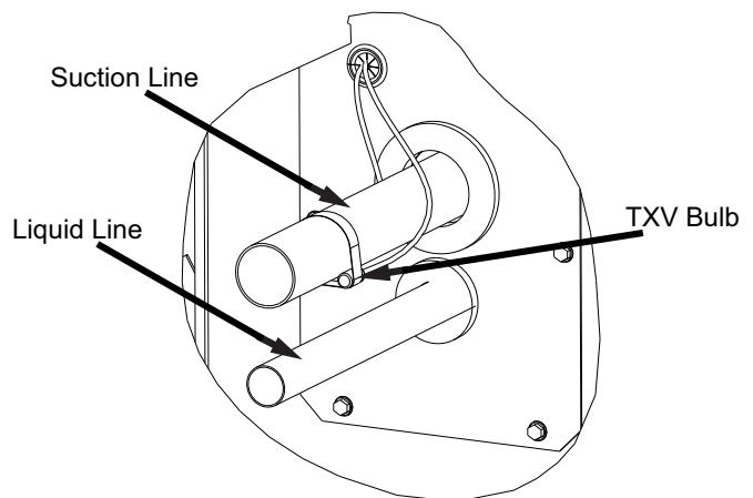
Figure 7: TVX Bulb Location
