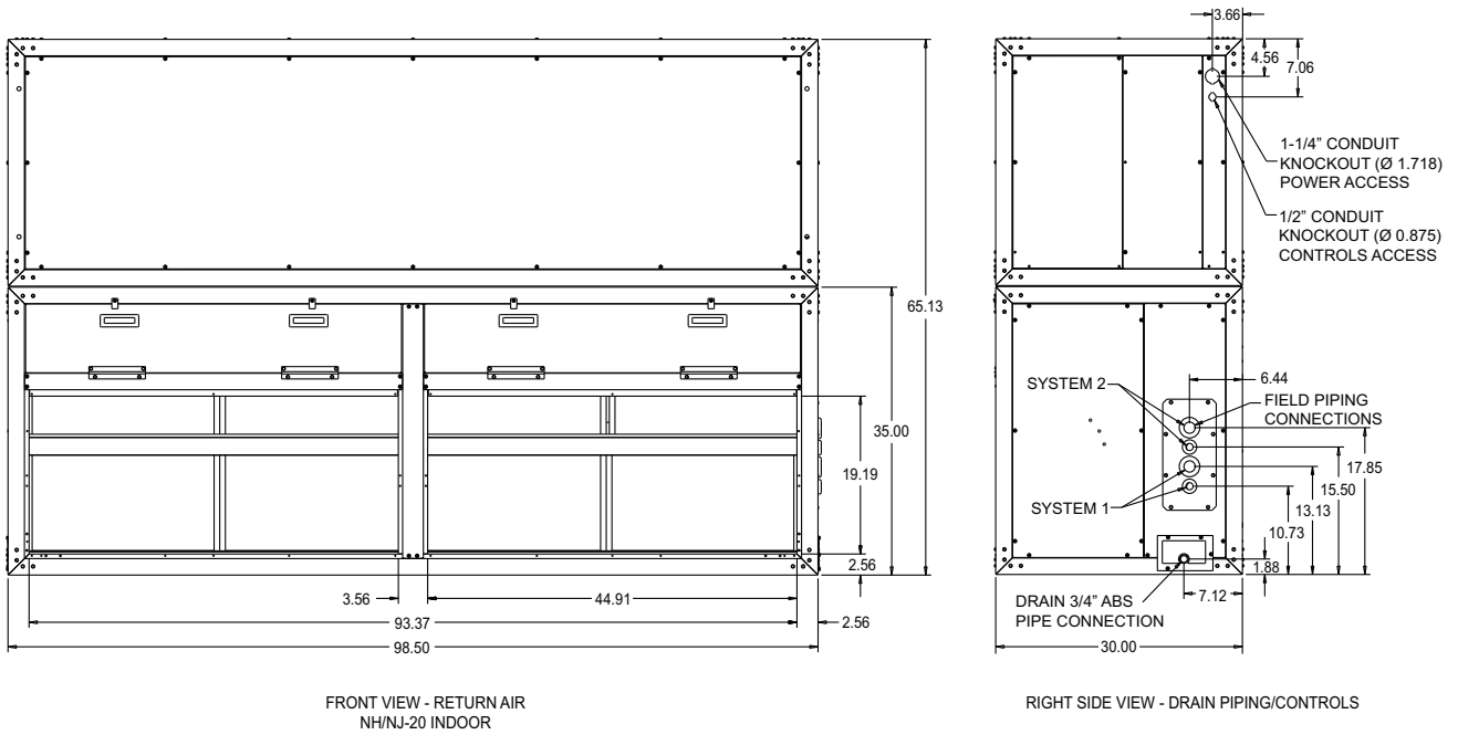
Figure 27: Unit Dimensions NH/NJ-20
