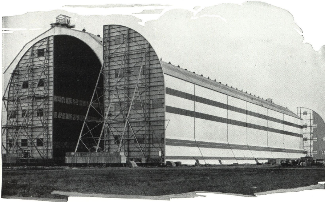
UNITED STATES GOVERNMENT BALLOON HANGAR, SCOTT FIELD, ILL. Erection supervised by Construction Quartermaster.
