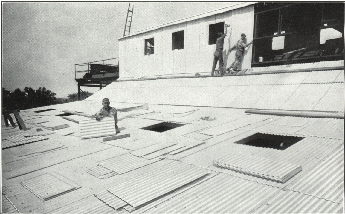
This building of the Iowa Southern Utilities Company, Centerville, Iowa, will be free from roof troubles practically as long as the structure stands. The natural gray surface of this Transite Corrugated Asbestos Roofing never needs paint or other protective coating. David F. Fisher & Co., Engineers.
