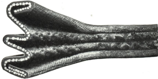
Cross-section of Coil Style No. 33, end opened to show construction.
