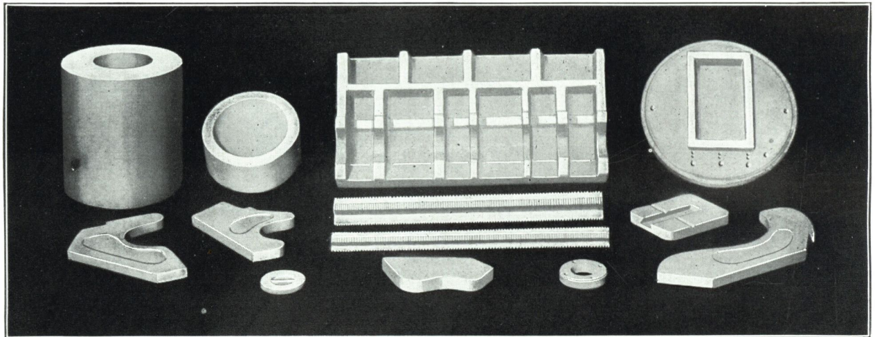
Heat proof cores, arc defectors, apparatus bases moulded of Electrobestos give greater security at less expense. Electrobestos is chemically inert, of high dielectric and mechanical strength and heat-resisting.
