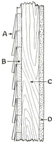
Construction No. 1
