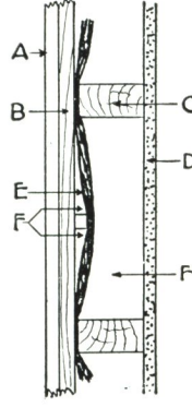
Construction No. 3
