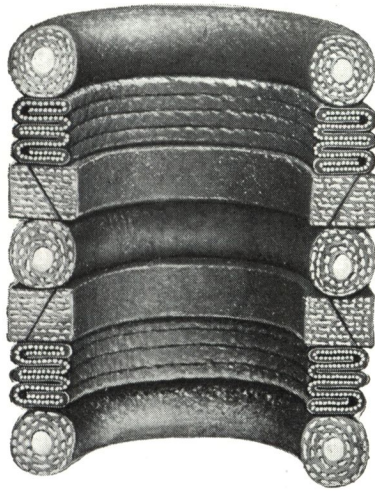
Universal Combination Ring, Style No. 29
