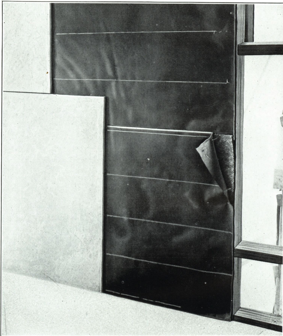
The above photograph shows Housline installed between the walls of one of the buildings at the Edgewater Plant of the Warner Sugar Refining Company. This is the ideal construction where the conservation of heat is essential in skeleton frame buildings.
