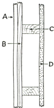
Construction No. 1
