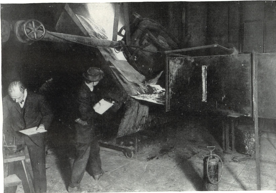
FIG. 1—MAKING RADIANT HEAT TEST
