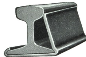
Transmission rail of the Elevated and the New York Subway. The exposed parts covered by indurated fibre material.
