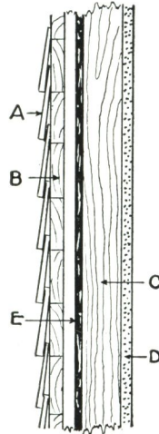
Construction No. 3
