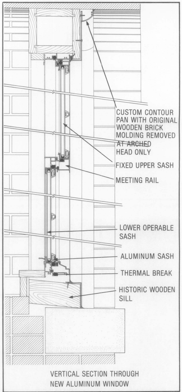
Figure 5. Vertical section of both the original wooden window and the replacement aluminum window. Drawings: Penelope Watson
