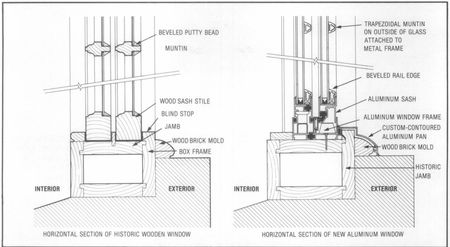
Figure 3. Horizontal section of both the original wooden window and the replacement aluminum window. Drawings: Penelope Watson
